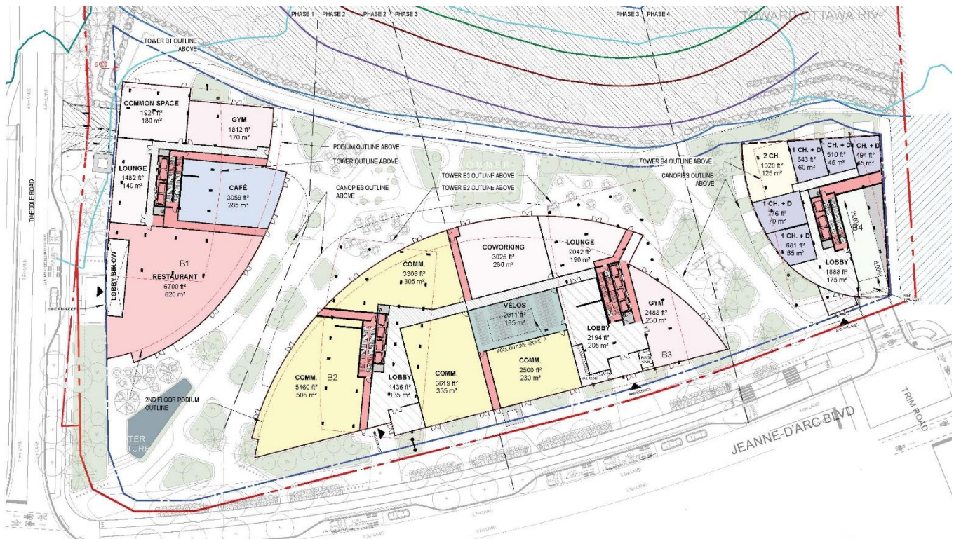
Figure 11: Ground Floor Plan (Neuf Architects)
