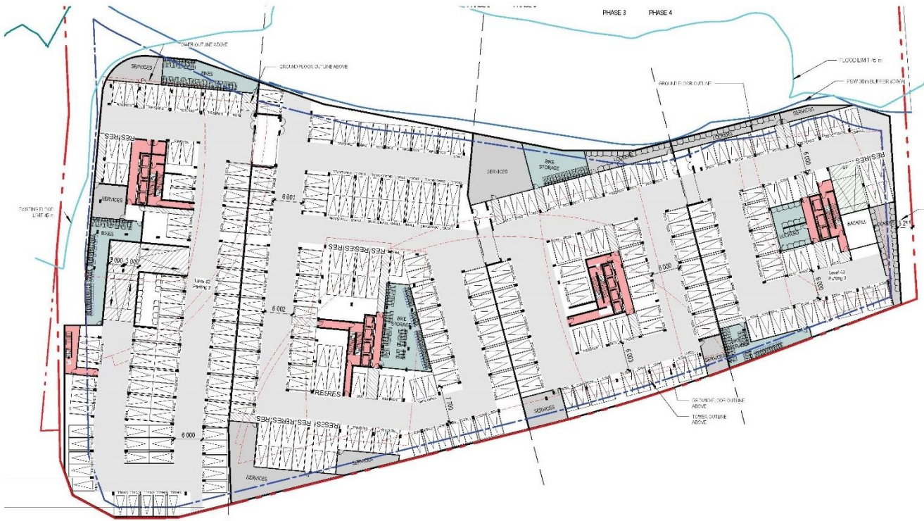
Figure 17: P3 Parking Plan (NEUF Architects)
