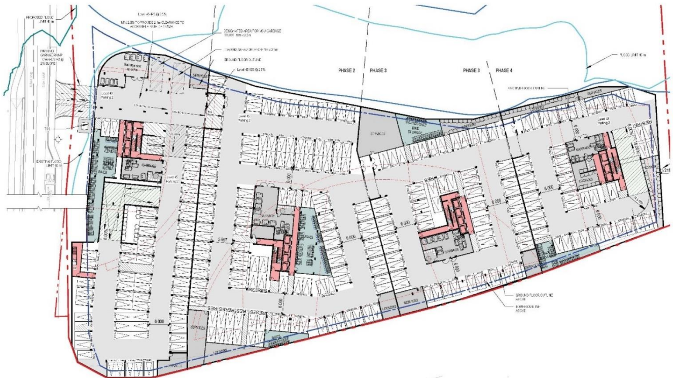
Figure 16: P2 Parking Plan (NEUF Architects)
