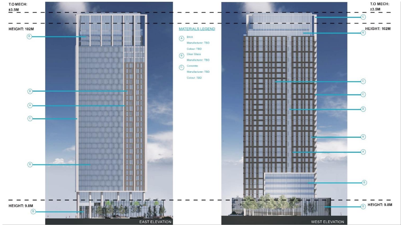
Figure 22: East and West Elevations of Tower B2 (NEUF Architects)
