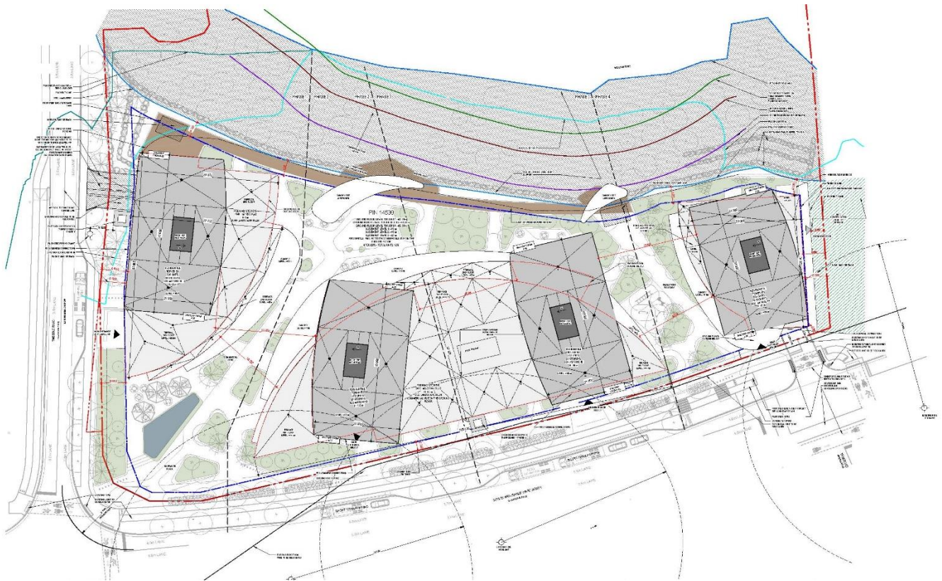
Figure 9: Site Plan (NEUF Architects)
