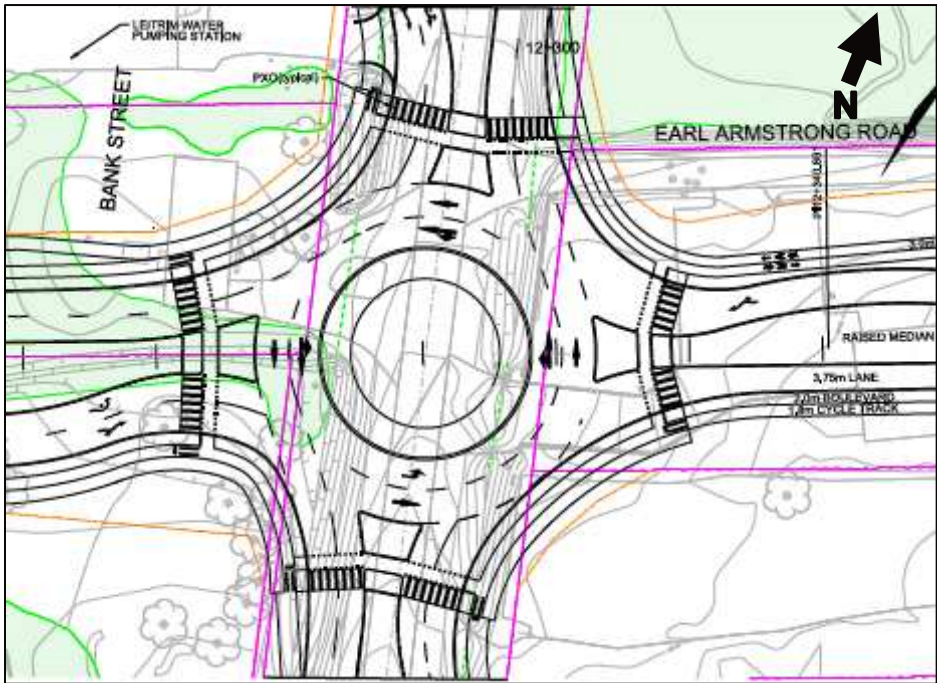
Figure 4-4 Future Bank Street & Earl Armstrong Road Roundabout
