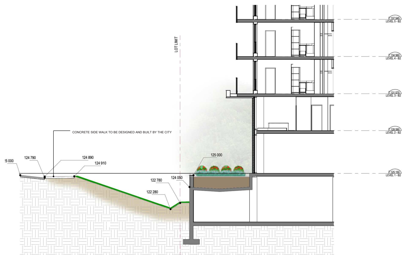
SECTION B
