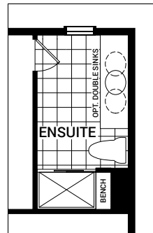
OPTIONAL ENSUITE 4' SHOWER W/ BENCH
