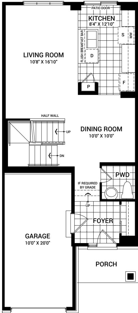
MAIN FLOOR PLAN B
