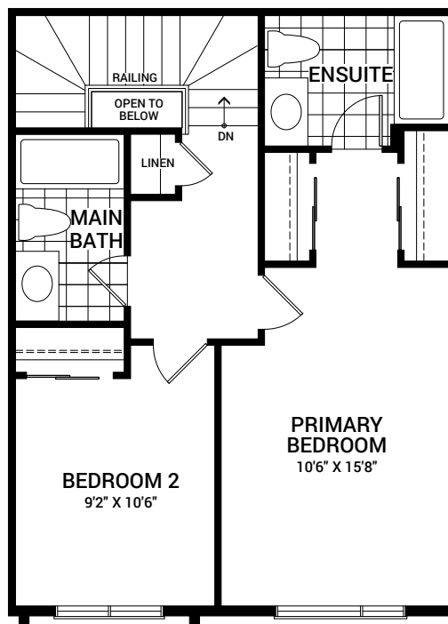
OPTIONAL THIRD FLOOR LAYOUT
