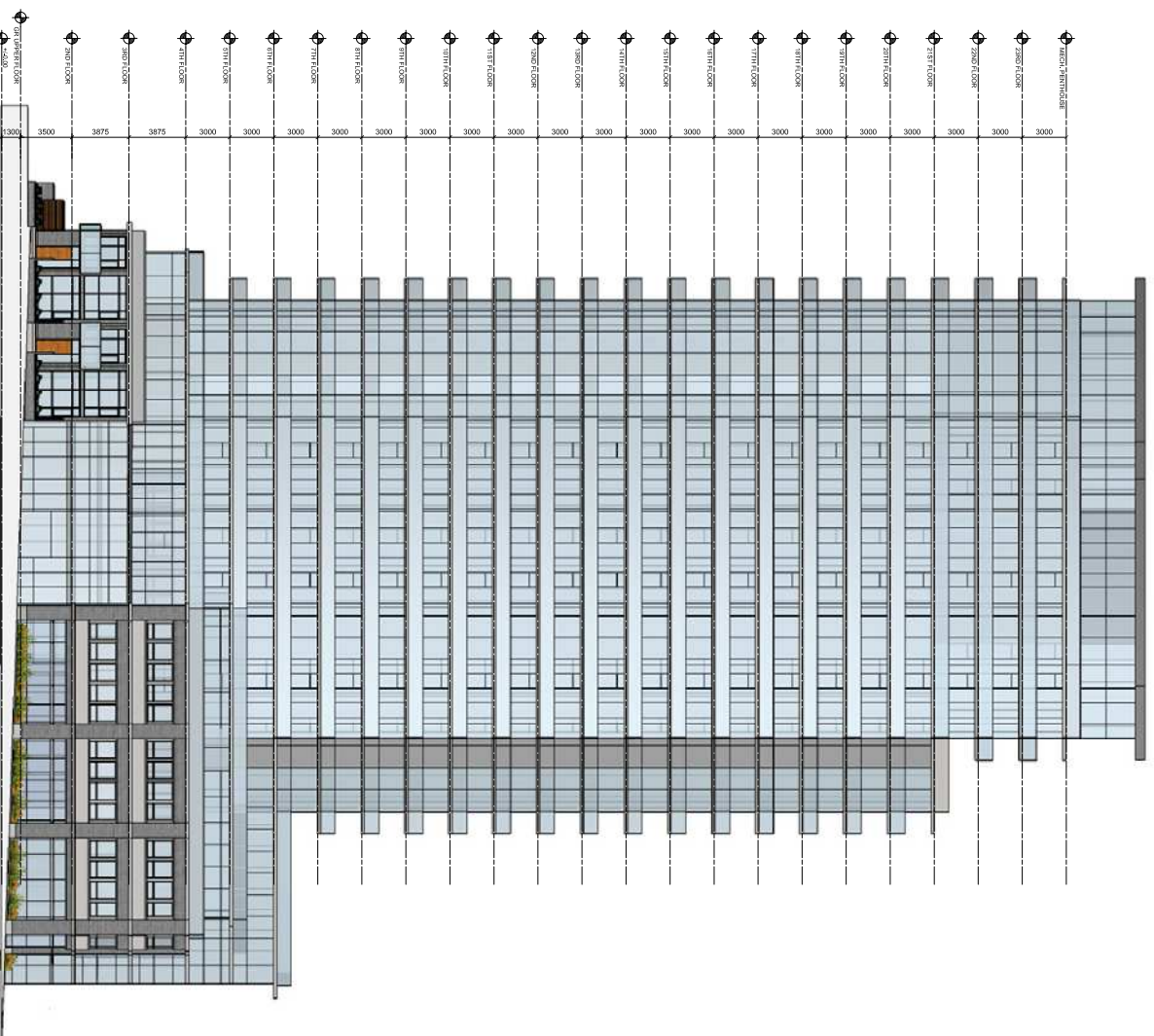
EAST ELEVATION
