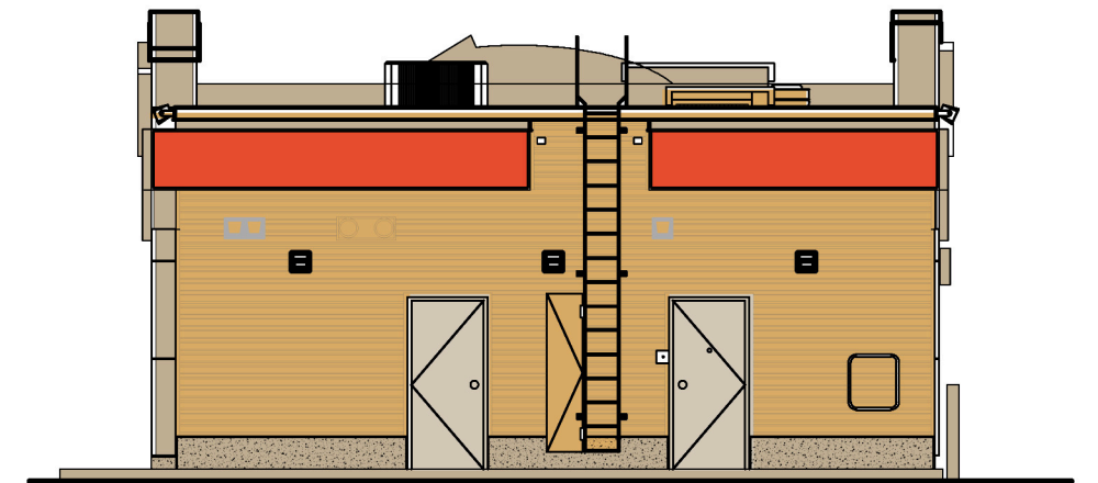
WEST ELEVATION
