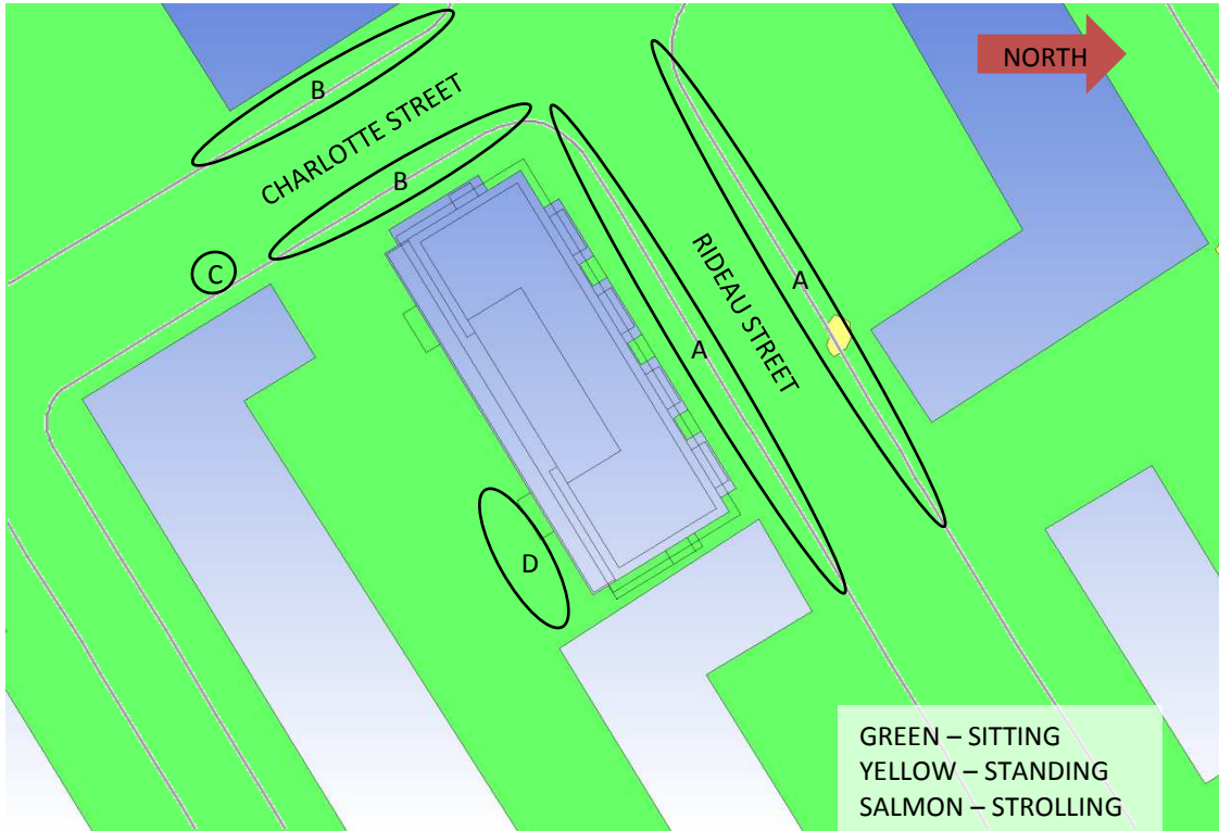
FIGURE 5A: AUTUMN – GRADE-LEVEL PEDESTRIAN WIND CONDITIONS
