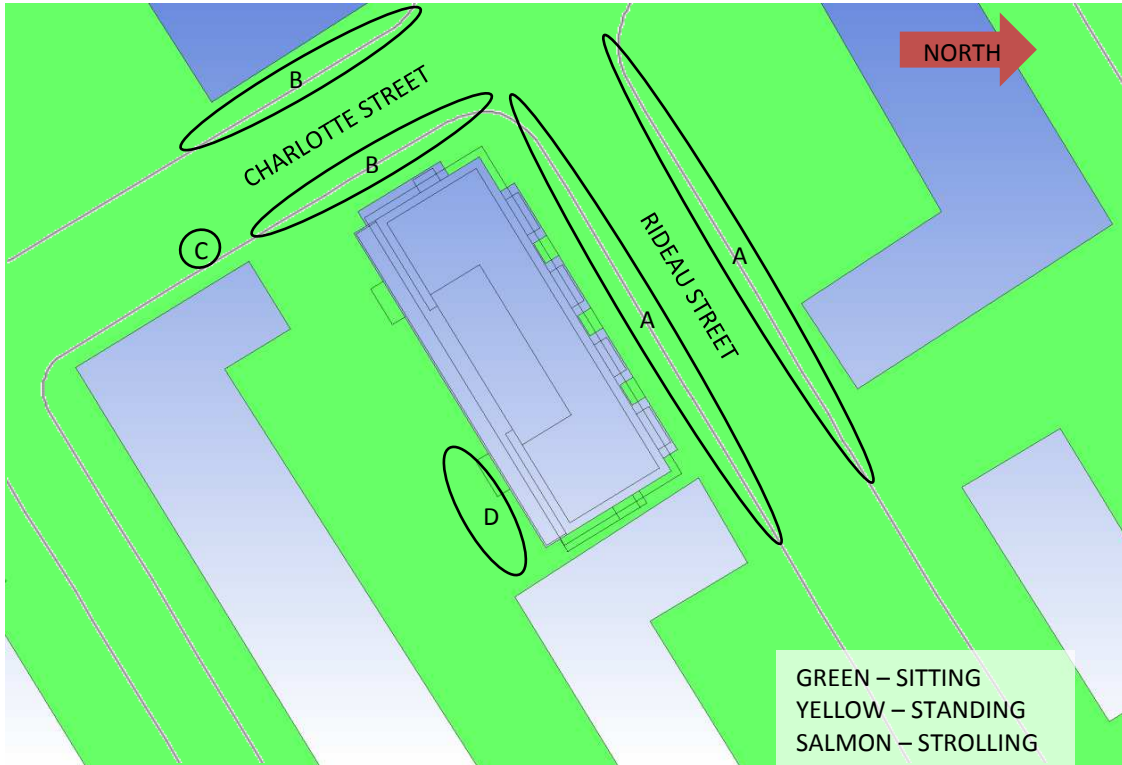
FIGURE 4A: SUMMER – GRADE-LEVEL PEDESTRIAN WIND CONDITIONS
