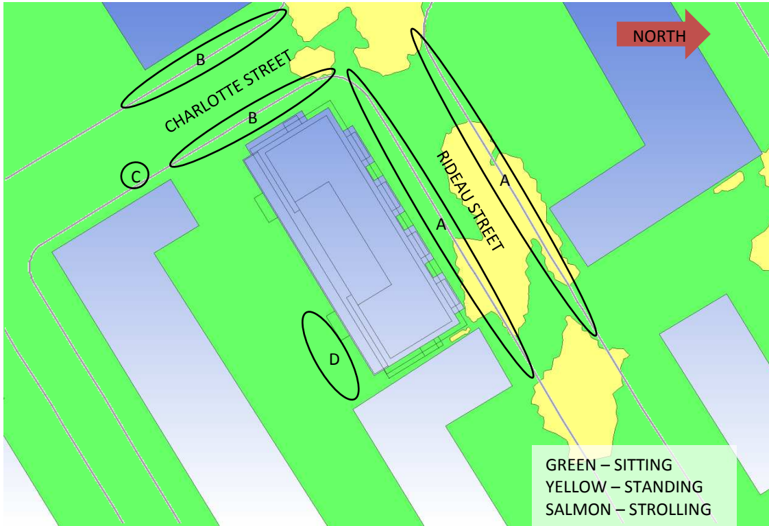
FIGURE 6A: WINTER – GRADE-LEVEL PEDESTRIAN WIND CONDITIONS
