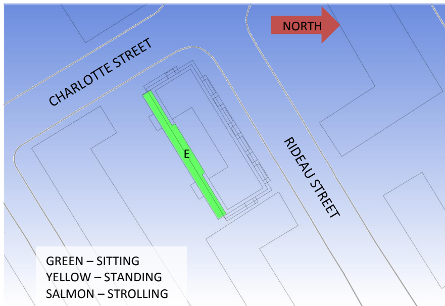
FIGURE 4B: SUMMER – LEVEL SEVEN AMENITY TERRACE PEDESTRIAN WIND CONDITIONS
