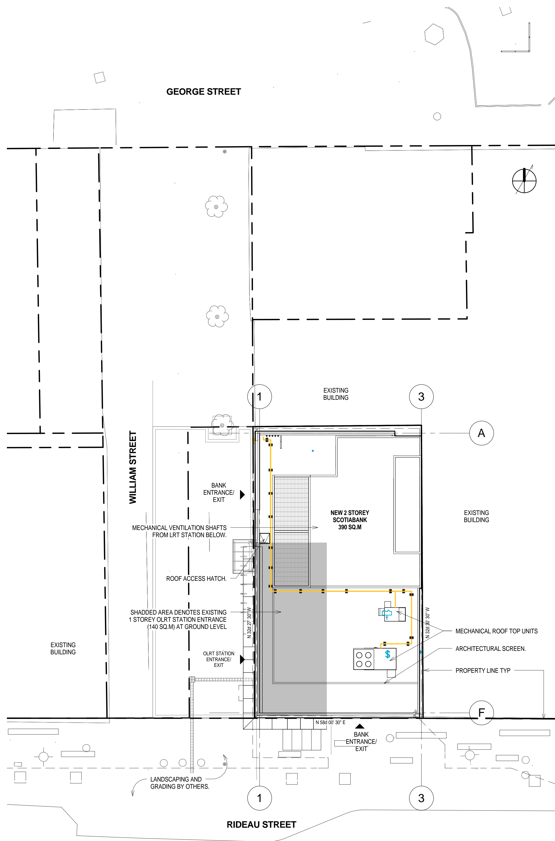
1 ARCHITECTURAL SITE PLAN A1000 1:200
