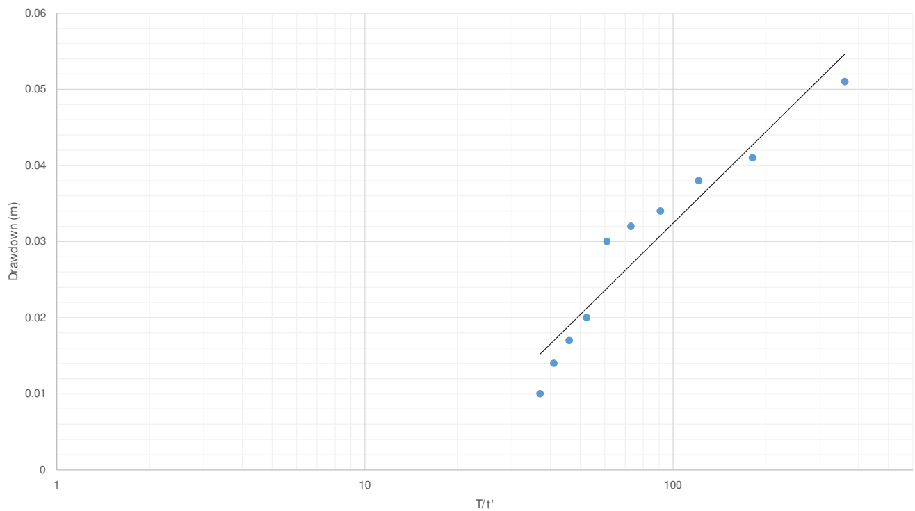
Drawdown (Recovery) vs Log Time 6688 Franktown Road, Ottawa, ON
