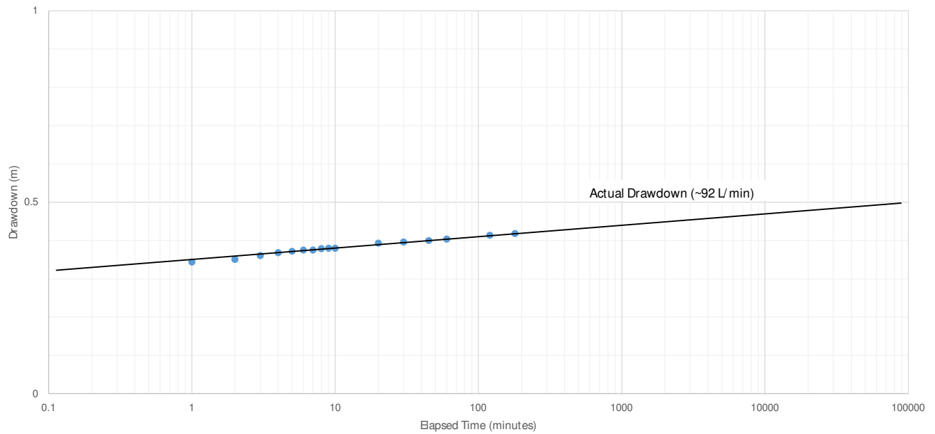
Drawdown vs Log Time TW1 Pumping Test (Drawdown), July 13, 2018 6688 Franktown Road, Ottawa, ON
