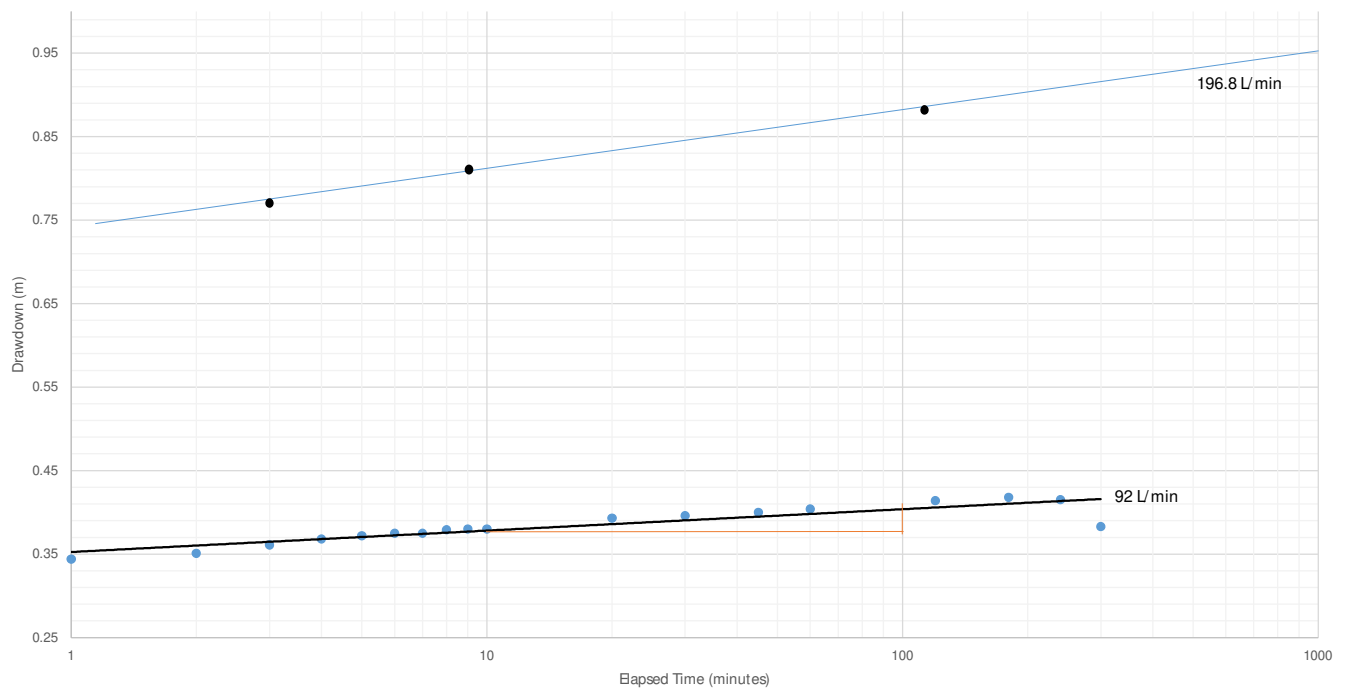
Drawdown vs Log Time TW1 Pumping Test (Drawdown), July 13, 2018 6688 Franktown Road, Ottawa, ON
