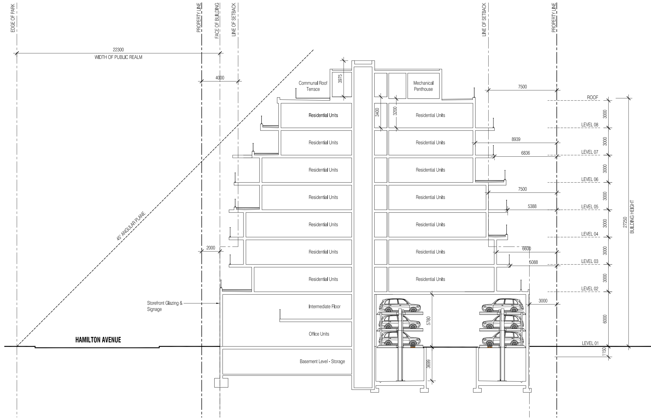
16 HAMILTON SECTIONAL STUDY SHOWING ANGULAR PLANE FROM RIGHT OF WAY
