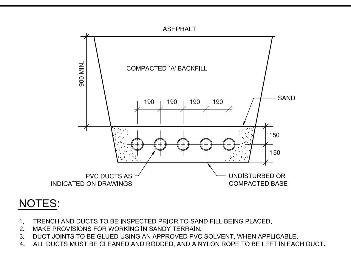
2 TYPICAL - DIRECT BURIED DUCT DETAIL E-01 N.T.S.
