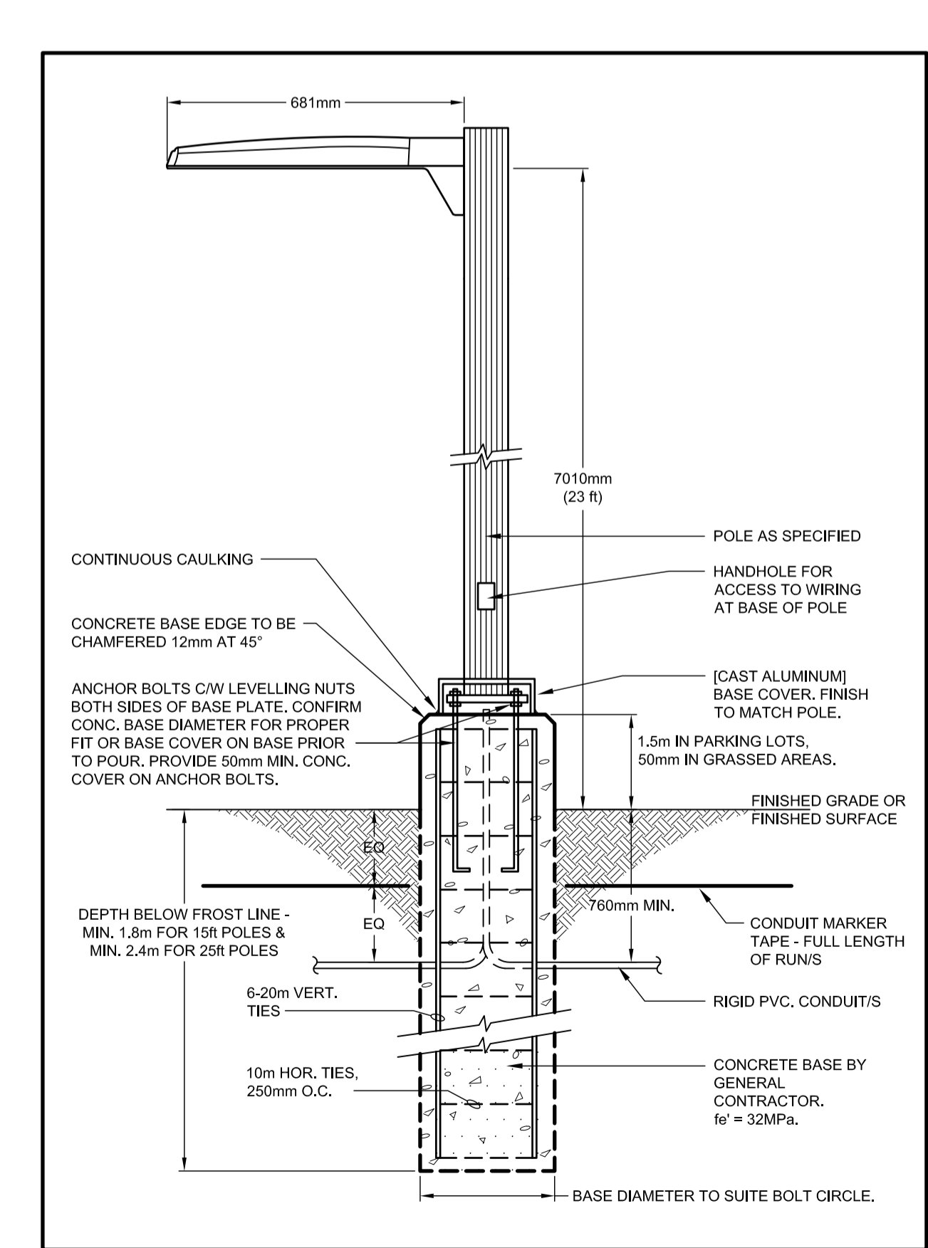
4 BASE DETAIL FOR POLE MOUNTED LUMINAIRES E-01 N.T.S.
