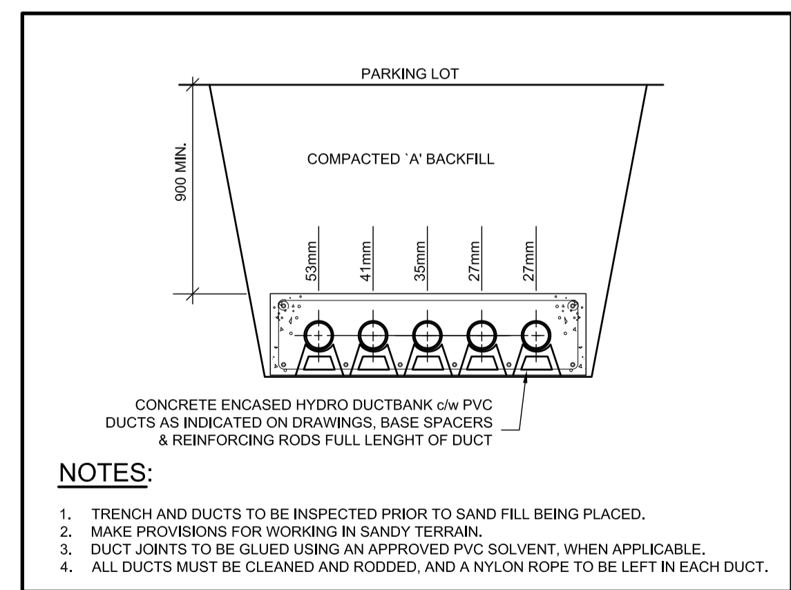
3 TYPICAL - DUCT DETAIL AT ROAD CROSSING E-01 N.T.S.
