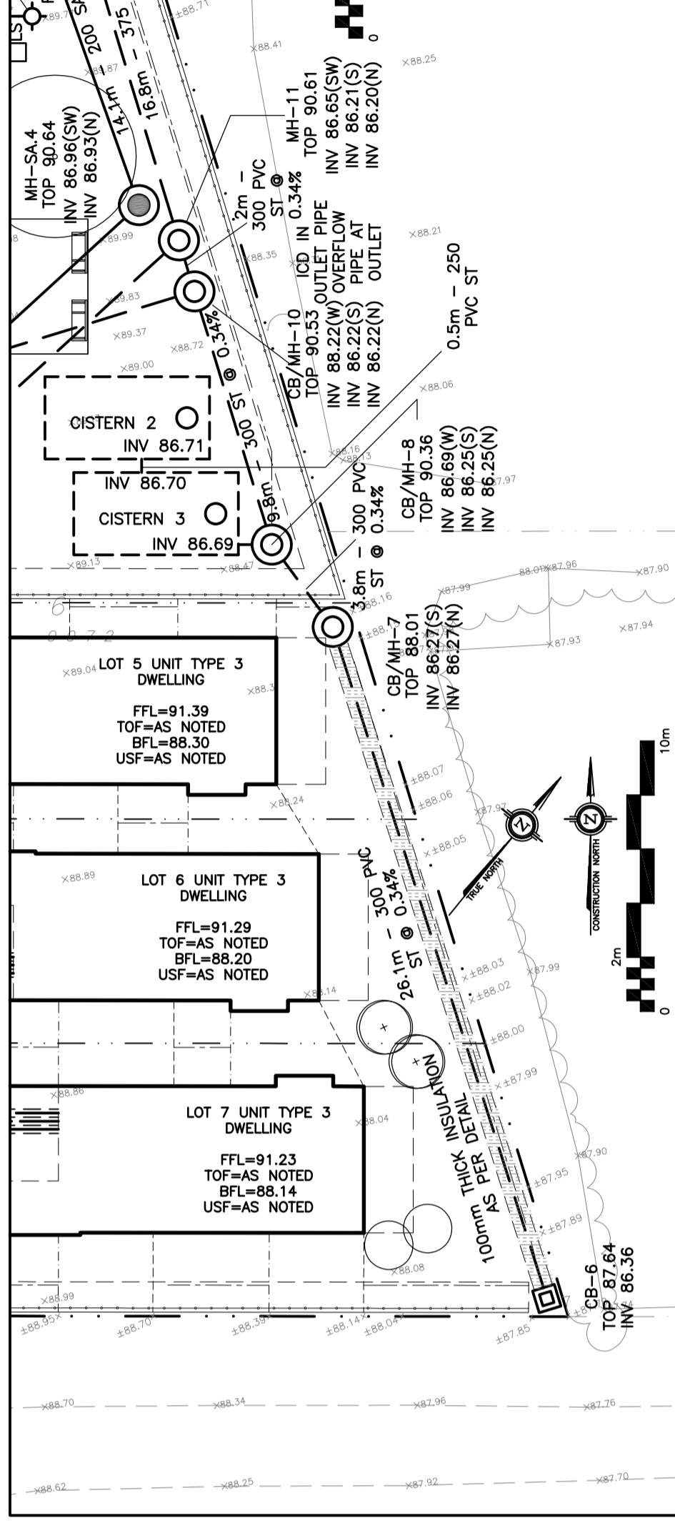
KEY PLAN
