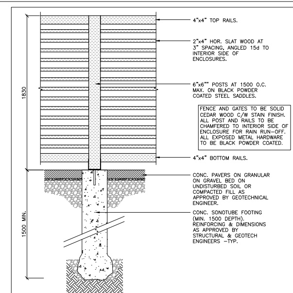
2 TYP. FENCE ENCLOSURE DETAIL A 105 1:20
