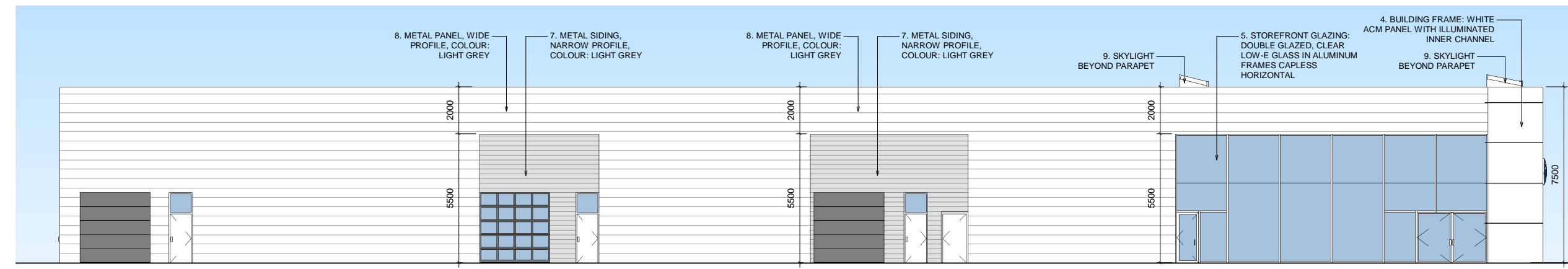
2 South 1 : 200
