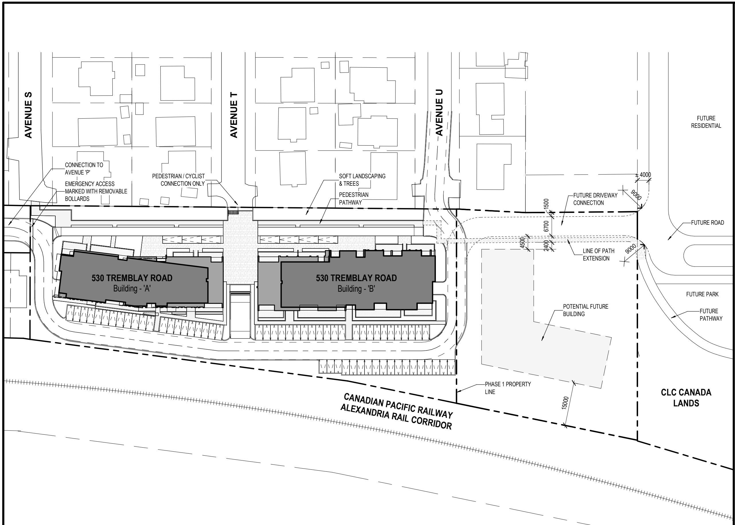
1 SITE PLAN SHOWING FUTURE PHASE AND CONNECTION TO CANADA LANDS ASK-01 SCALE: 1 : 750
