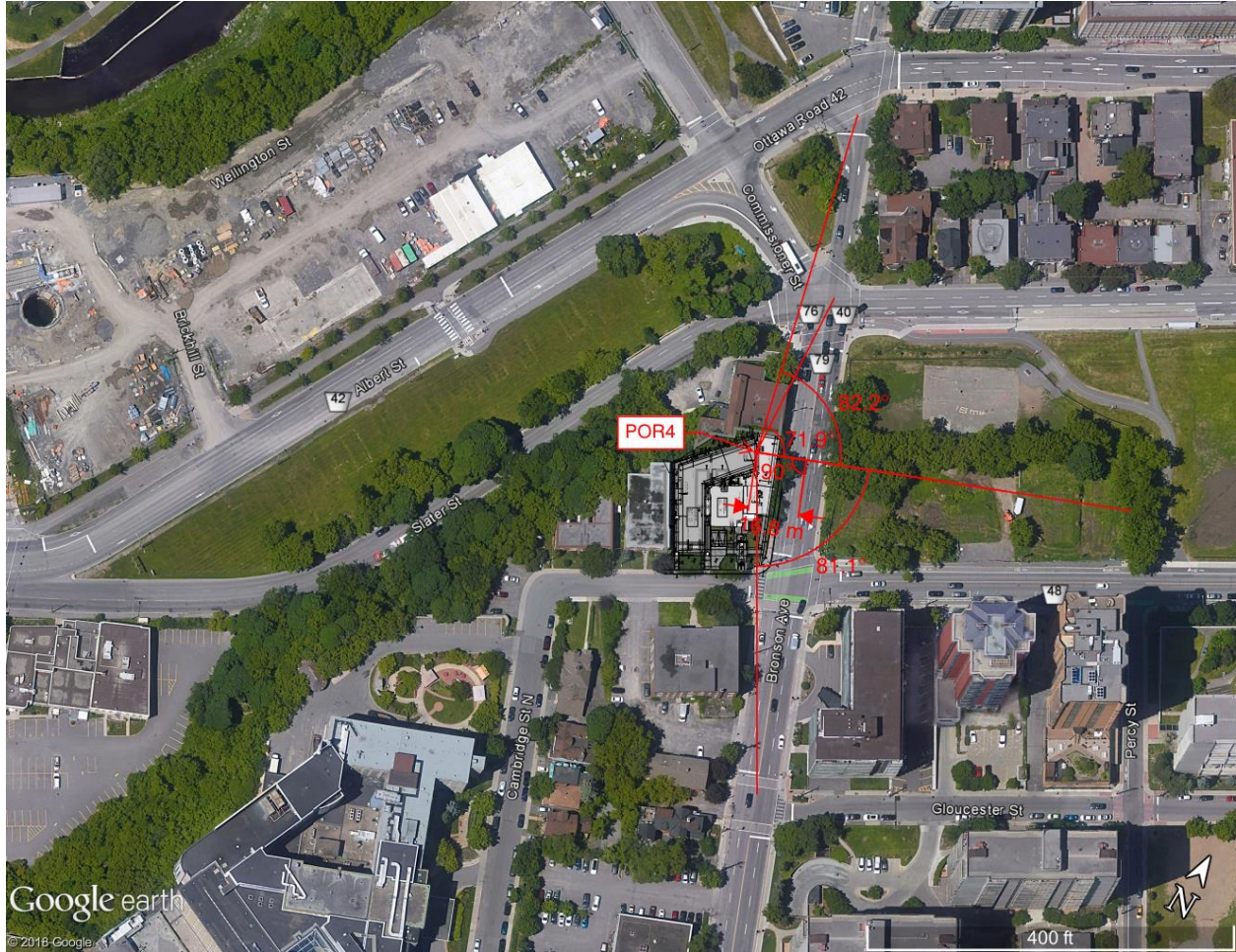
Figure 16: Distances and angles used in STAMSON 5.04 for POR4 (2 of 3)
