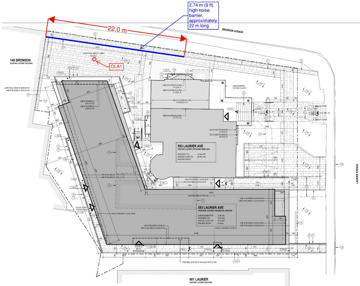
Figure 6: Proposed noise barrier location for OLA1
