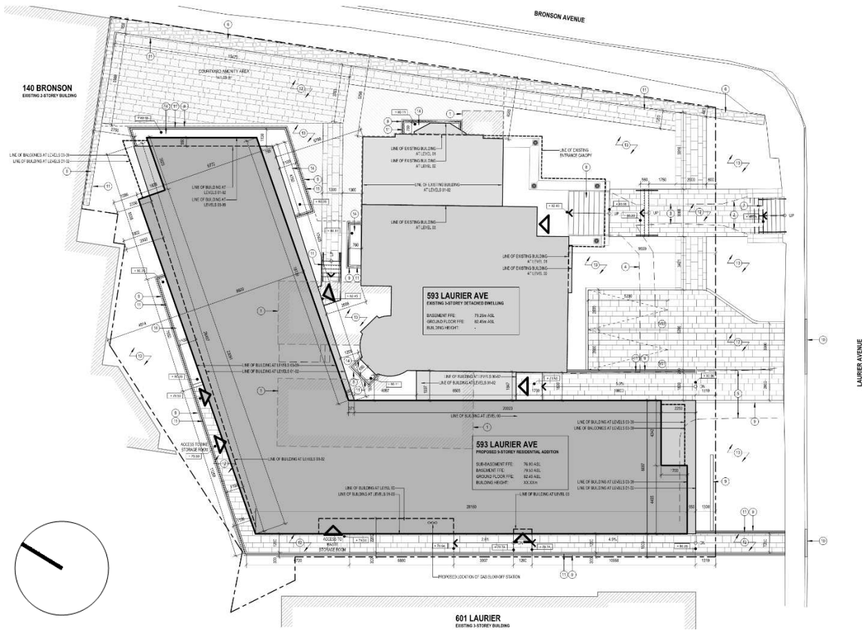
Figure 1: Site plan
