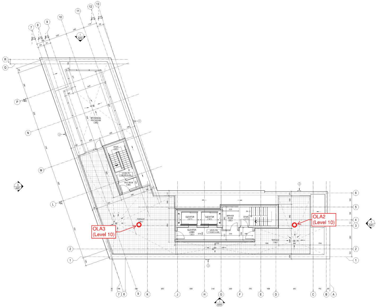
Figure 5: Outdoor living area (OLA2 and OLA3) locations
