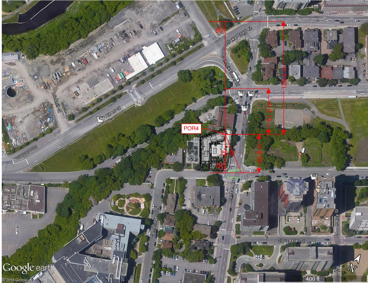
Figure 15: Distances and angles used in STAMSON 5.04 for POR4 (1 of 3)
