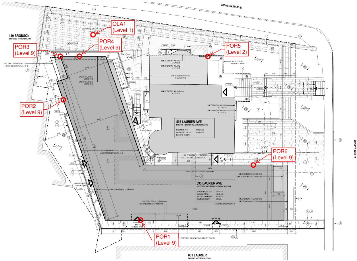
Figure 4: Point of reception (POR) and outdoor living area (OLA1) locations
