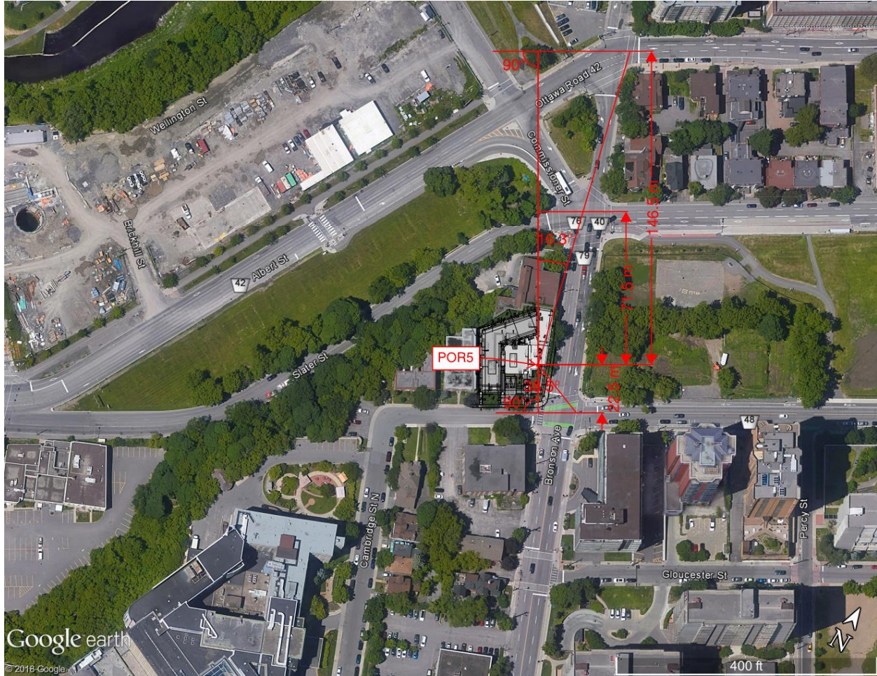
Figure 18: Distances and angles used in STAMSON 5.04 for POR5 (1 of 2)
