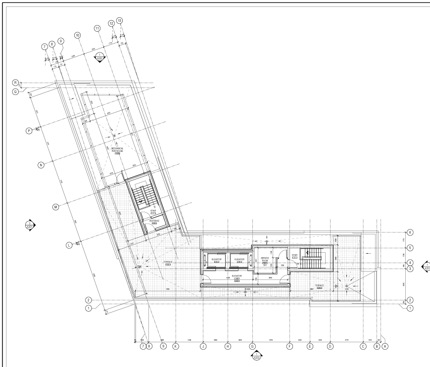
ROOF LEVEL - ROOF PLAN SCALE 1:75
