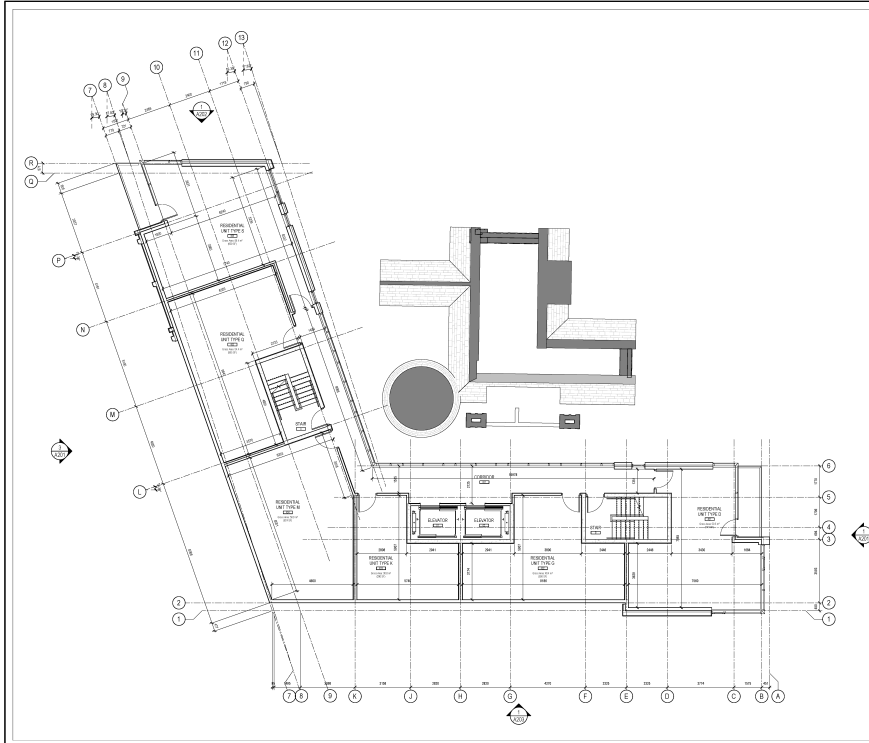
LEVEL 04 - FLOOR PLAN SCALE 1:75
