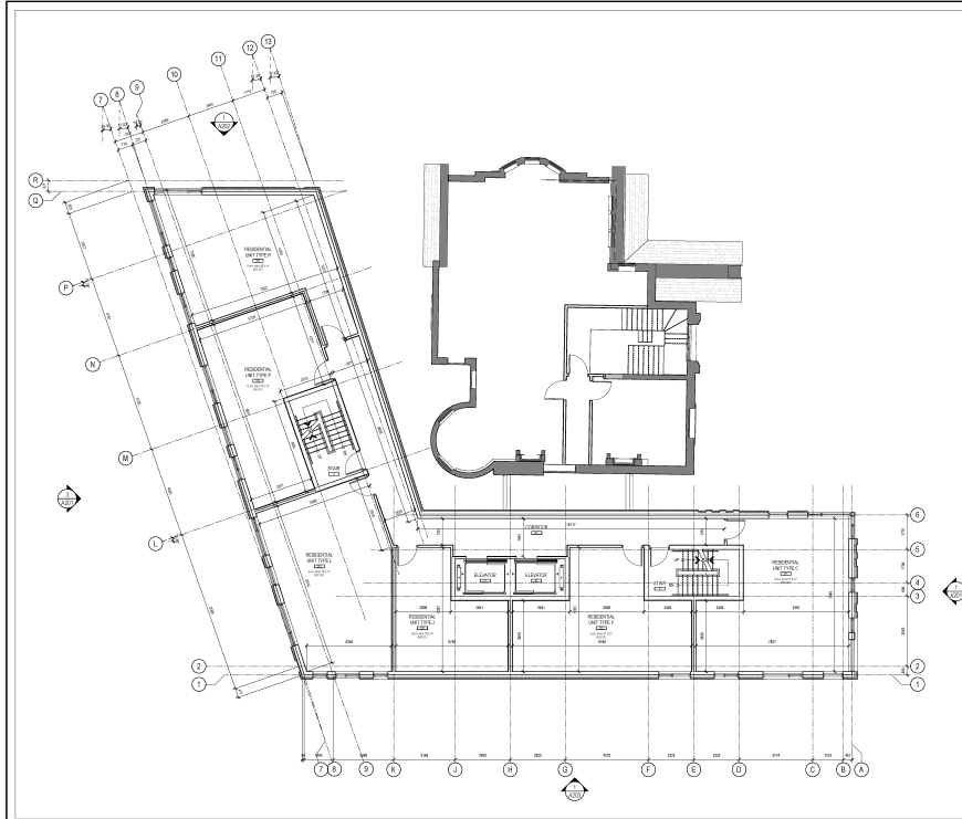
LEVEL 02 - FLOOR PLAN SCALE: 1:75
