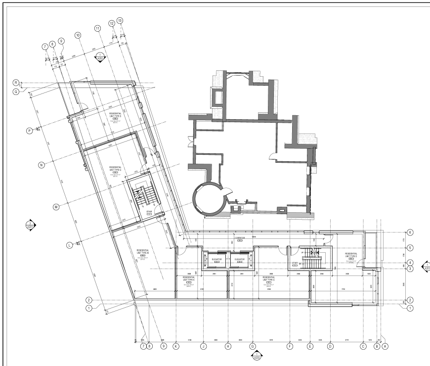
LEVEL 03 - FLOOR PLAN SCALE: 1:75
