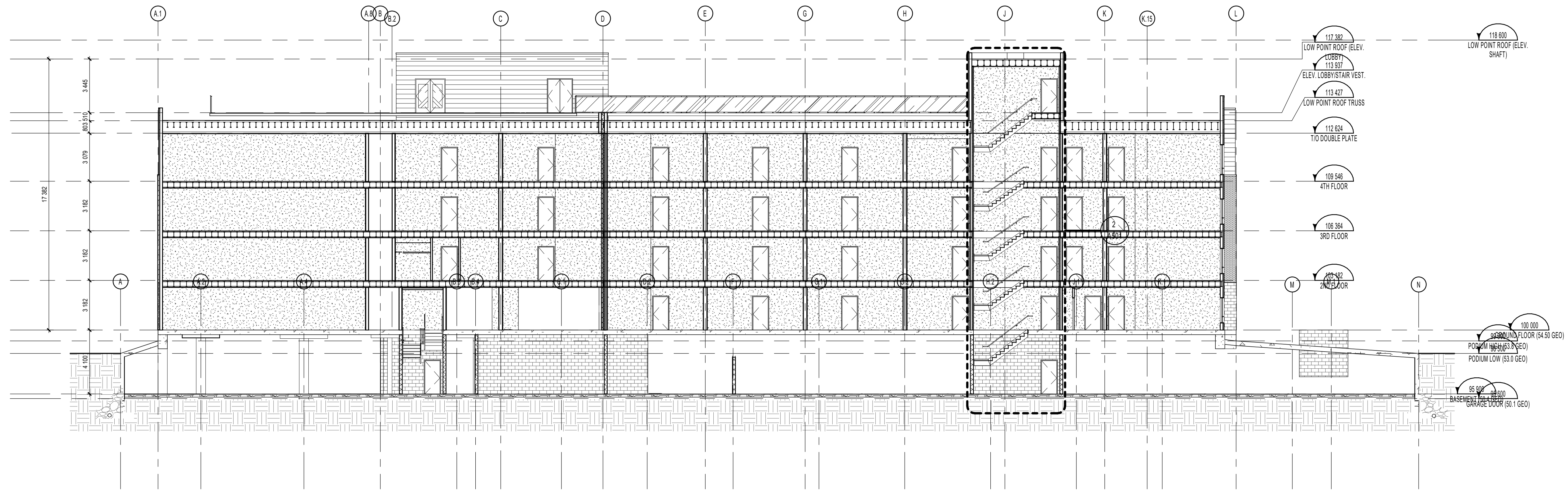
TRANSVERSAL OVERALL SECTION 2 1 : 150
