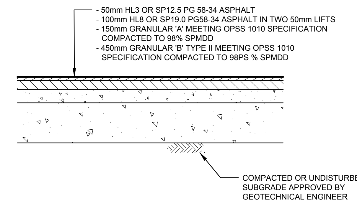
HEAVY DUTY PAVEMENT N.T.S.
