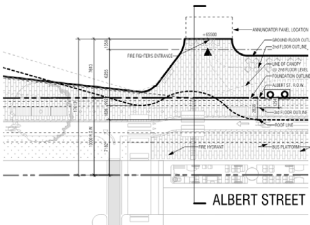
1 STREET SECTION - ALBERT ST. @ FIRE FIGHTER'S ENTRANCE A040 1:100
