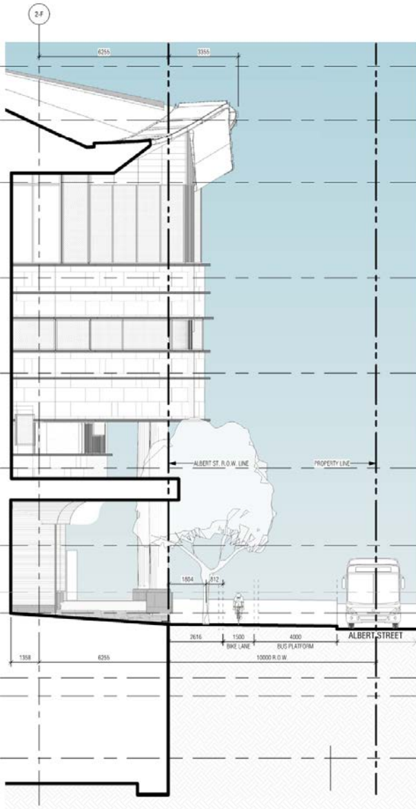
1 STREET SECTION - ALBERT ST. @ FIRE FIGHTER'S ENTRANCE A040 1:100
