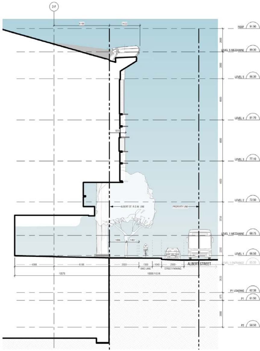
5 STREET SECTION - ALBERT ST. @ FIREFIGHTER'S ENTRANCE ROAD 1:100
