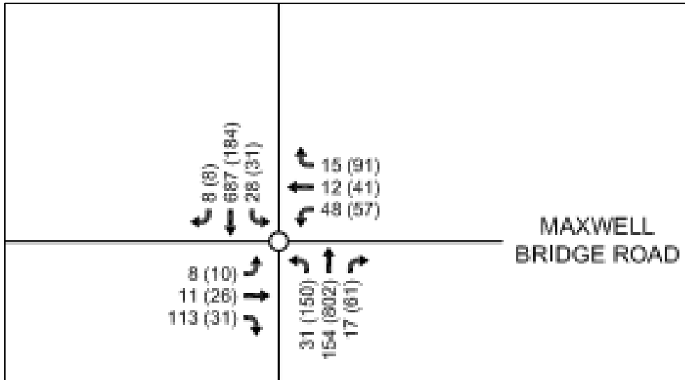
Figure 14: Kanata North Community Design Plan - 2026 Future Background Volumes
