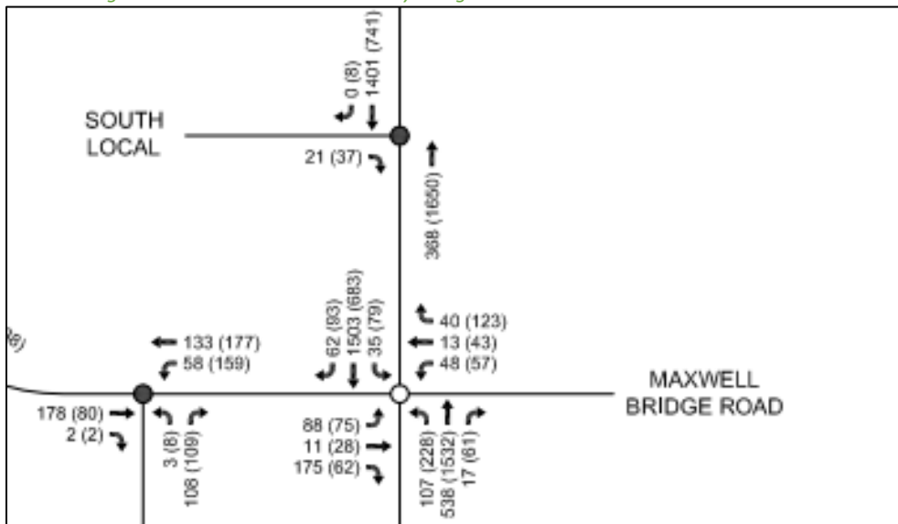
Figure 15: Kanata North Community Design Plan - 2026 Future Total Volumes
