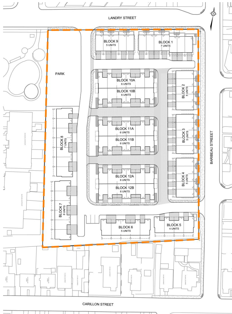
Figure 2: Site Plan
