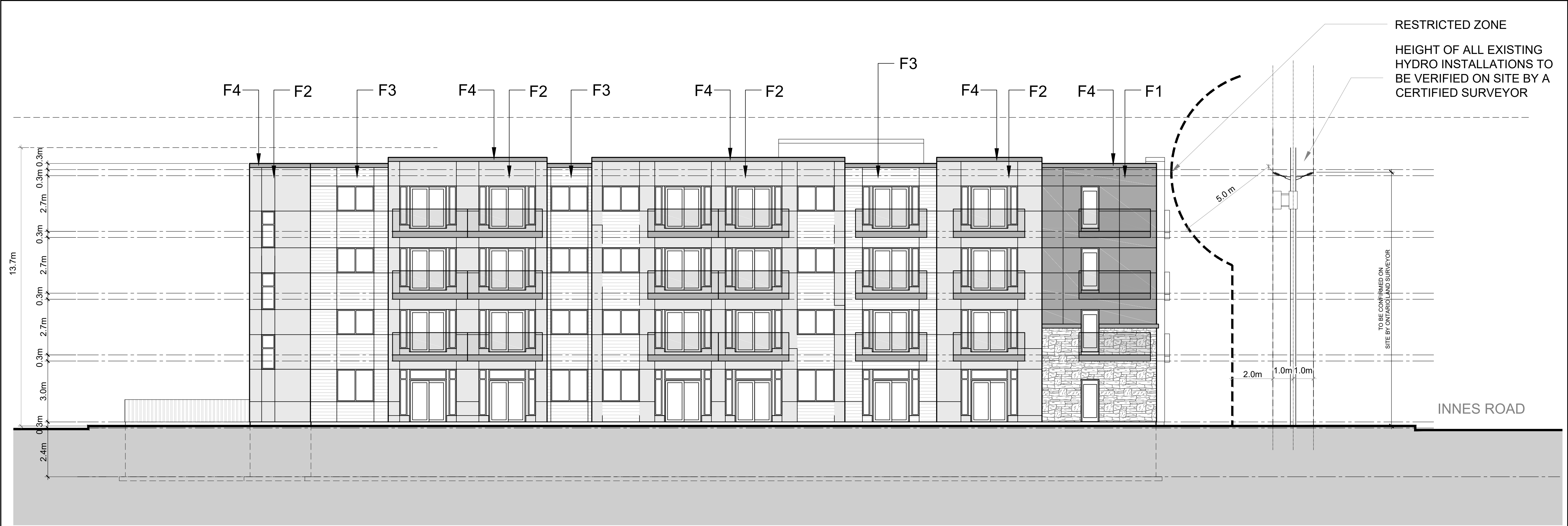
4 BLOCK A WEST ELEVATION (BLOCK B MIRRORED) SCALE: 1:100
