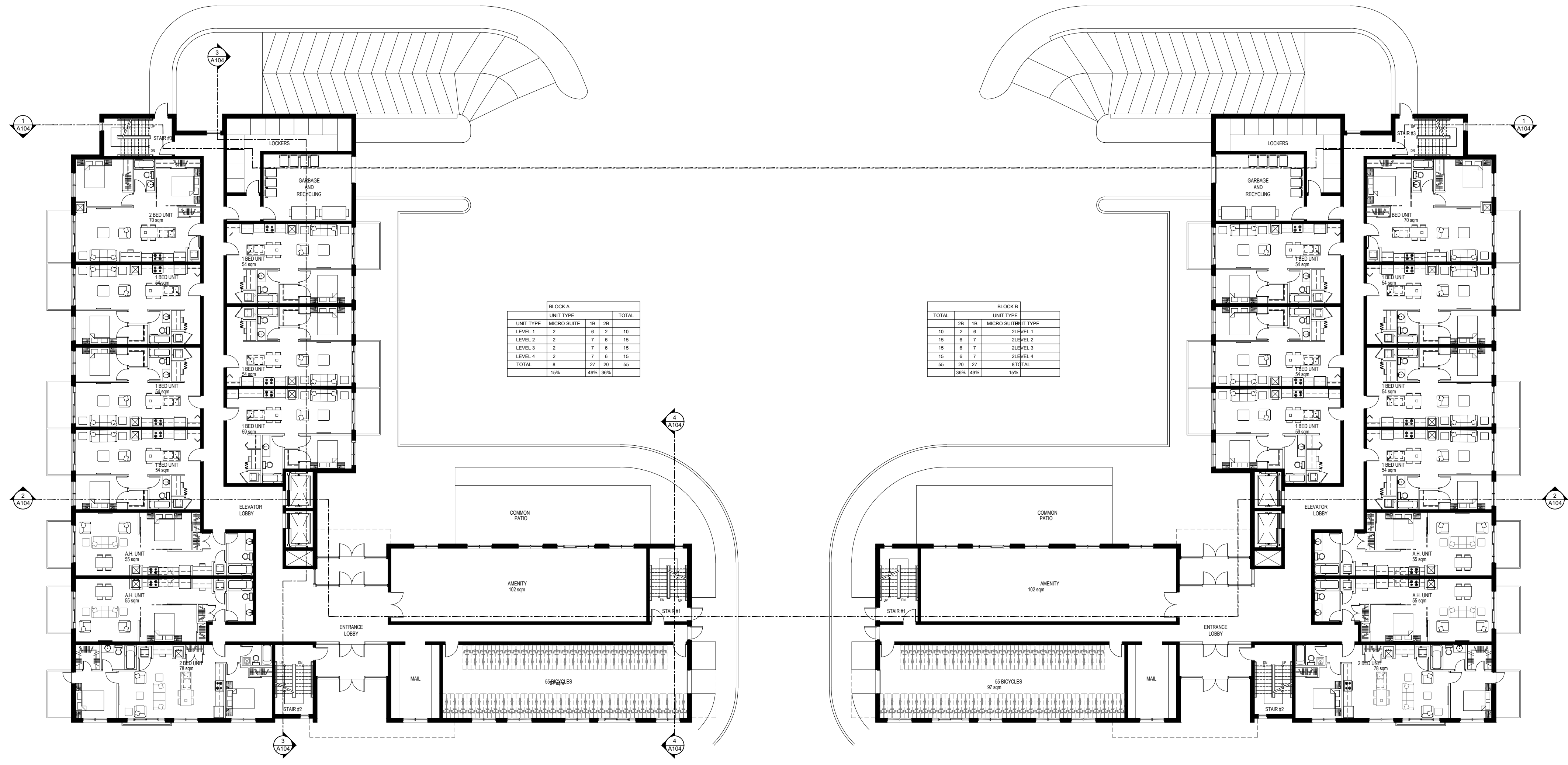
1 MAIN LEVEL PLAN SCALE = 1 : 200
