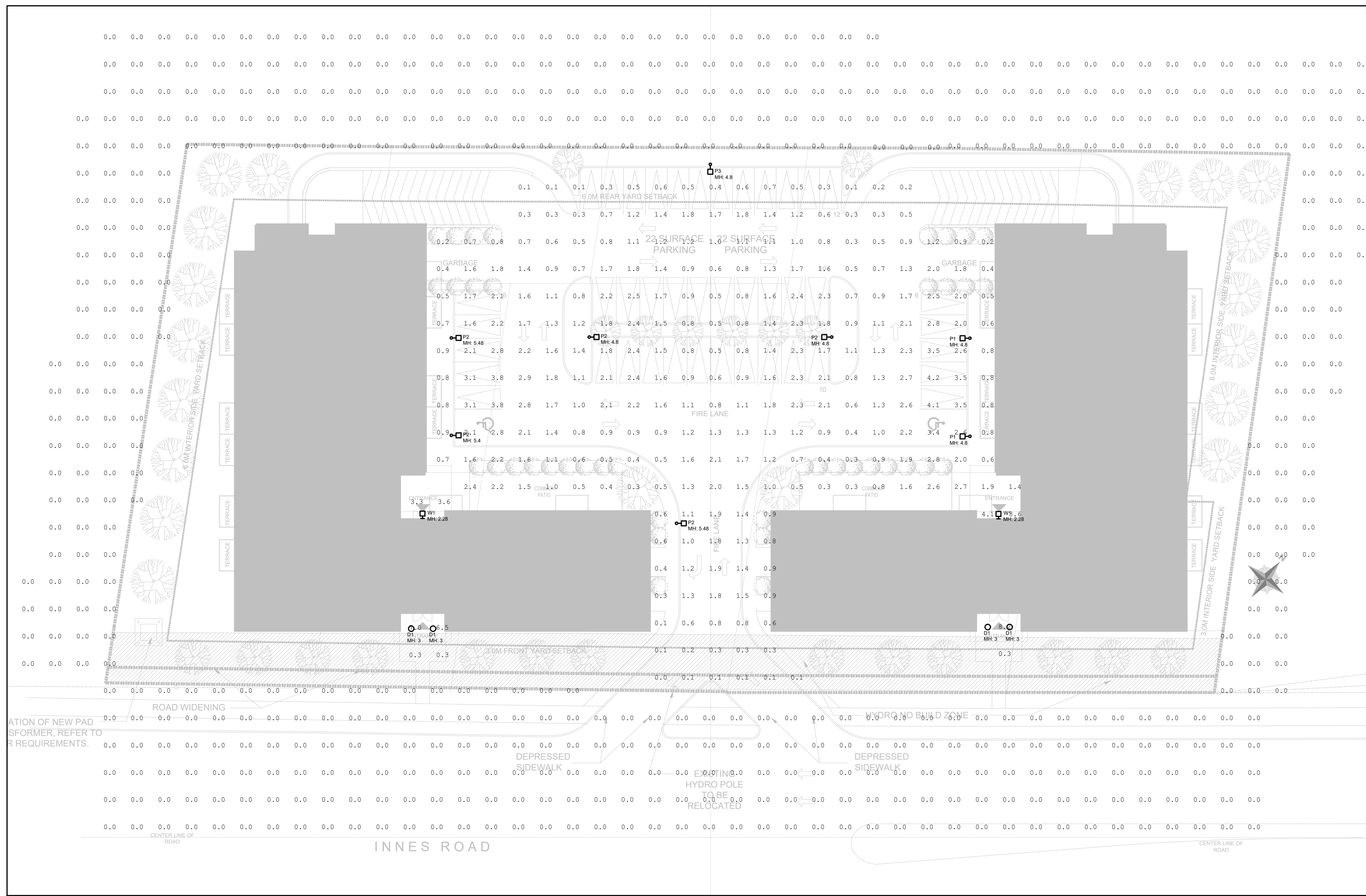
1 ELECTRICAL SITE PLAN SCALE: 1:250
