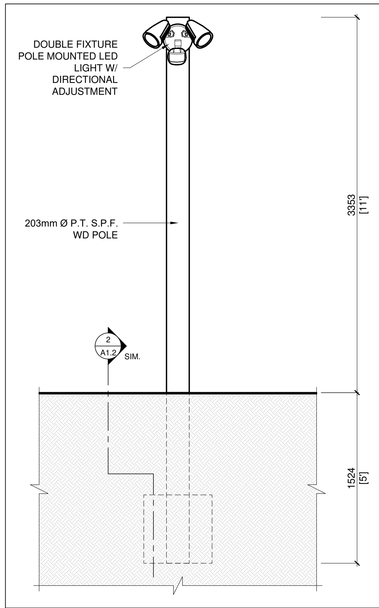
1 LIGHT POLE A1.3 1:20
