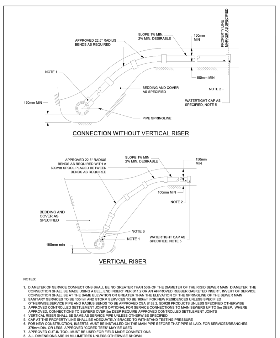
SEWER SERVICE CONNECTIONS FOR RIGID MAIN SEWER PIPE (MODIFIED OPSD-1006.010)
