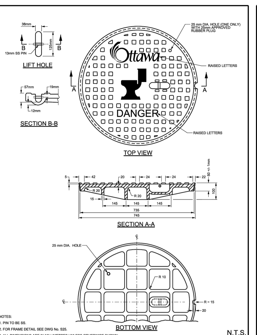
STANDARD CIRCULAR SANITARY & COMBINED MAINTENANCE HOLE COVER
