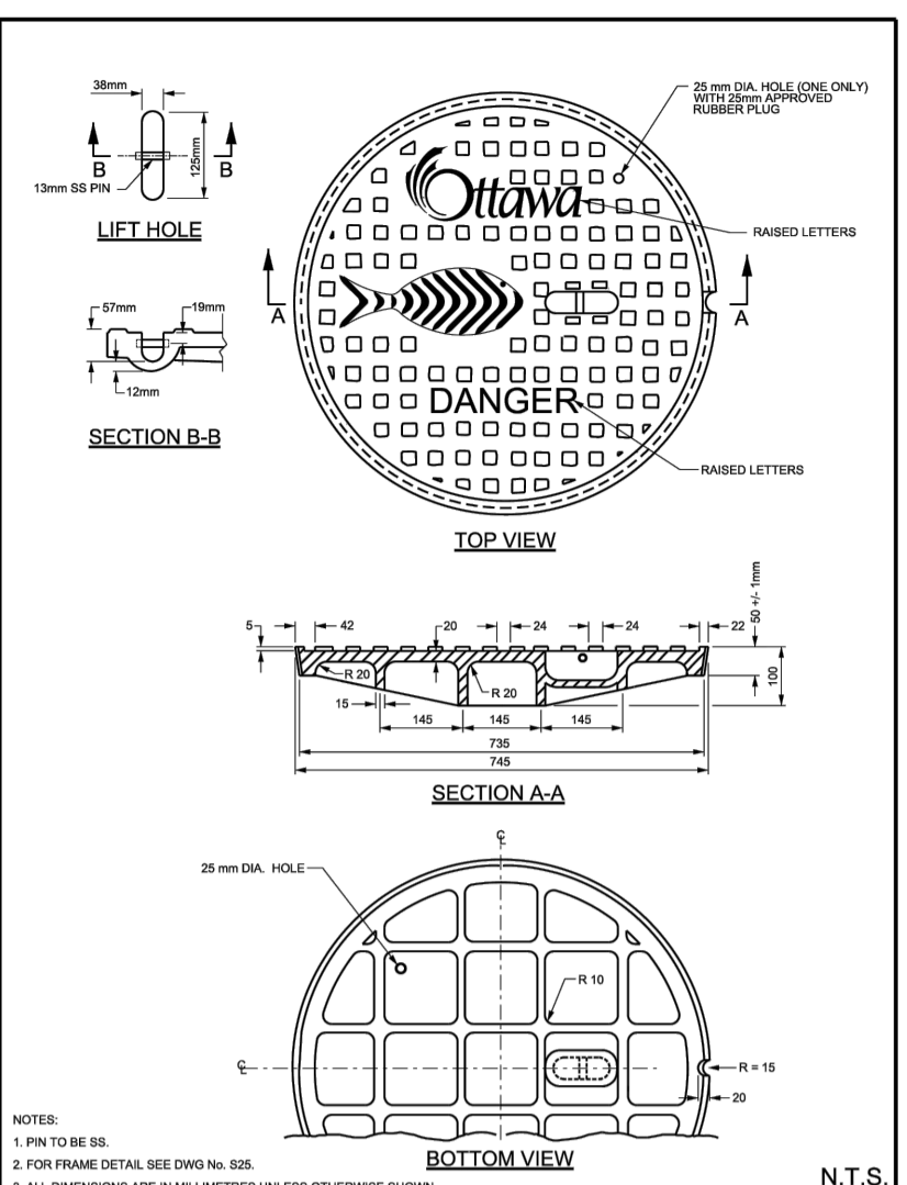
STANDARD CIRCULAR STORM MAINTENANCE HOLE COVER
