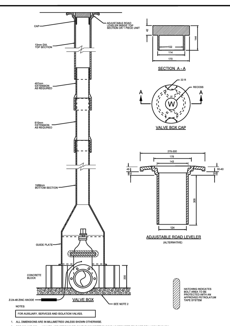
VALVE BOX ASSEMBLY
