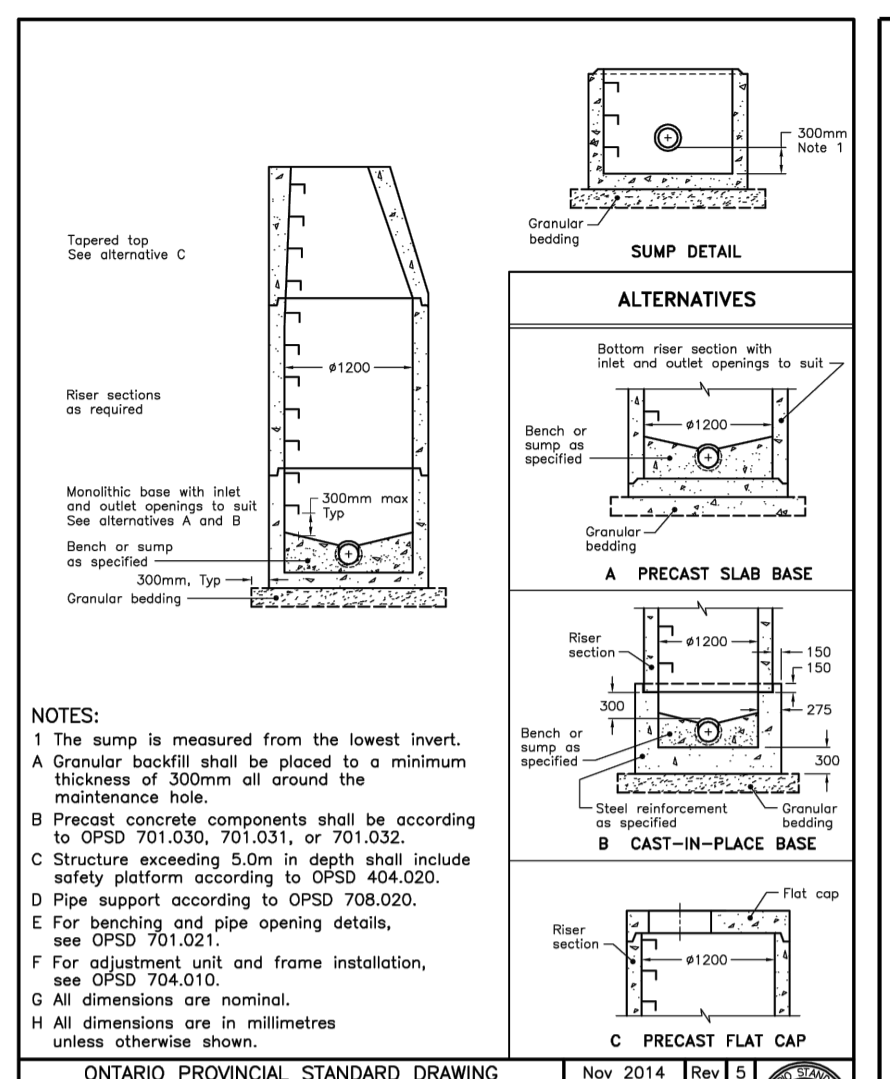
PRECAST CONCRETE MAINTENANCE HOLE 1200mm DIAMETER OPSD 701.010
