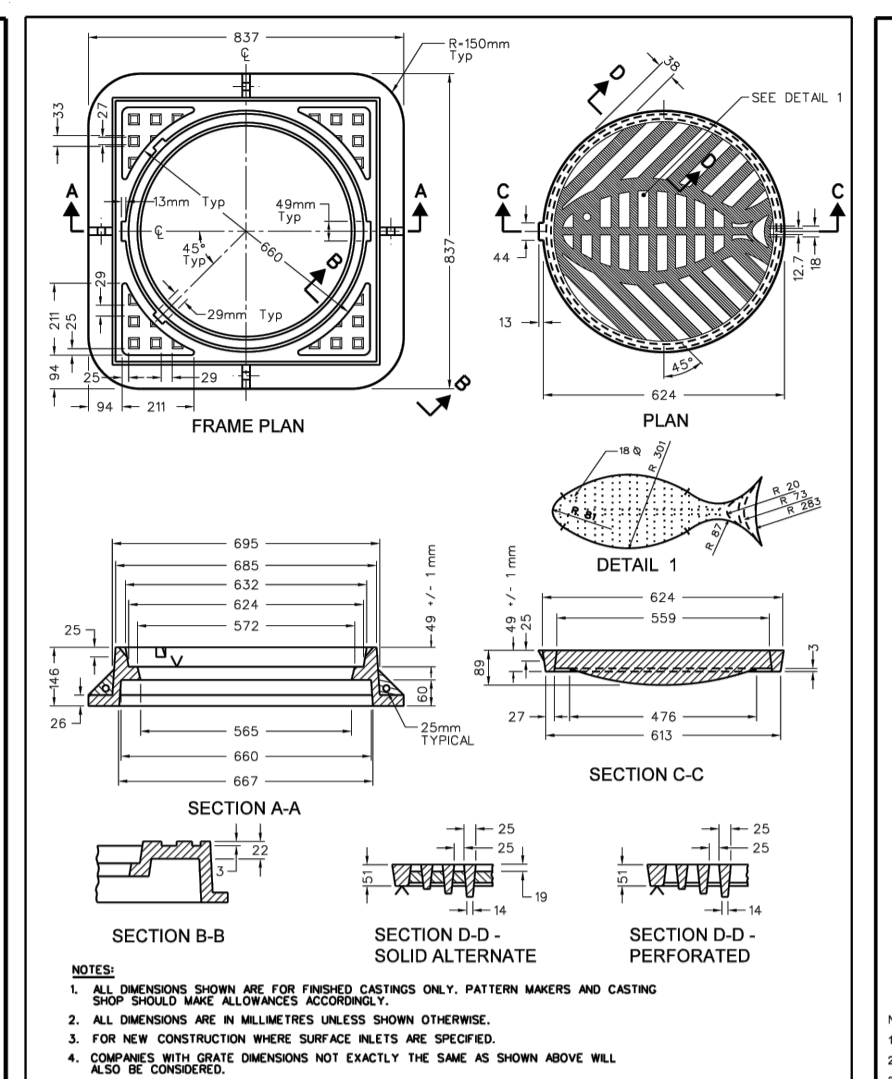
HEAVY DUTY "FISH" TYPE ROUND CATCH BASIN COVER (MODIFIED OPSD-400.07)
