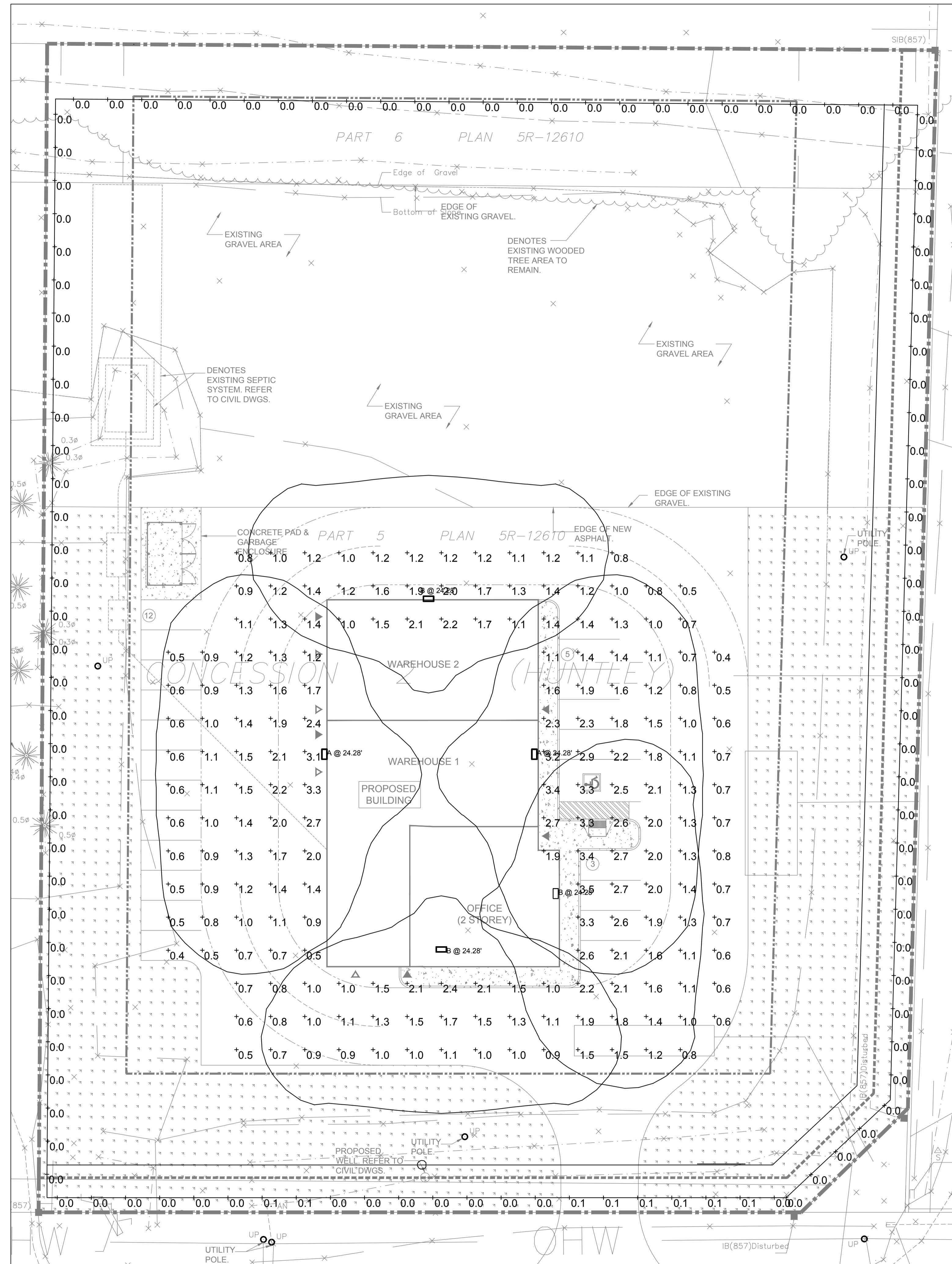
1 SITE LIGHTING PLAN E-1 1:200
