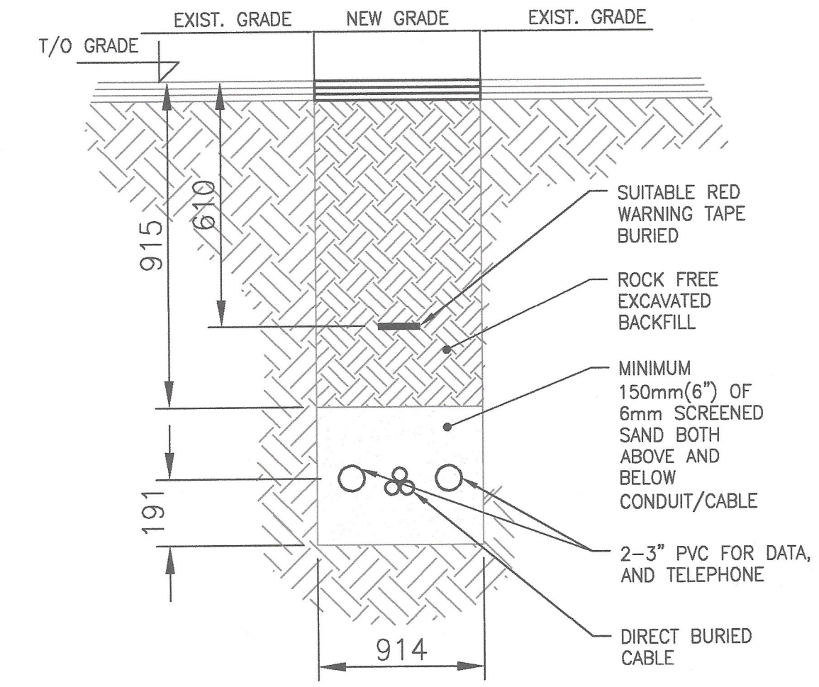
HYDRO SECONDARY TRENCH DETAIL (TYPICAL) SCALE NTS
