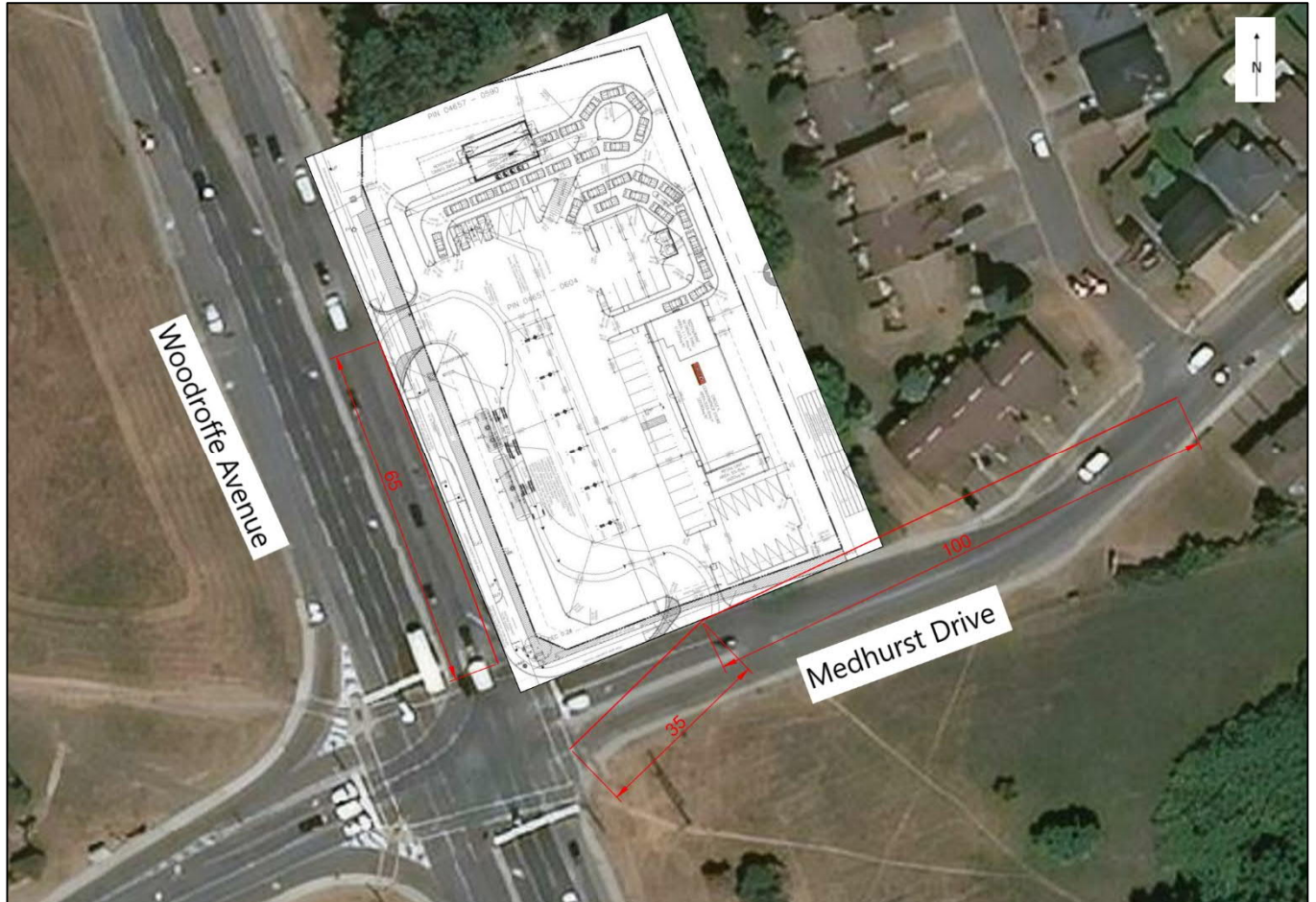
Figure 13.1 Accesses Sightlines
