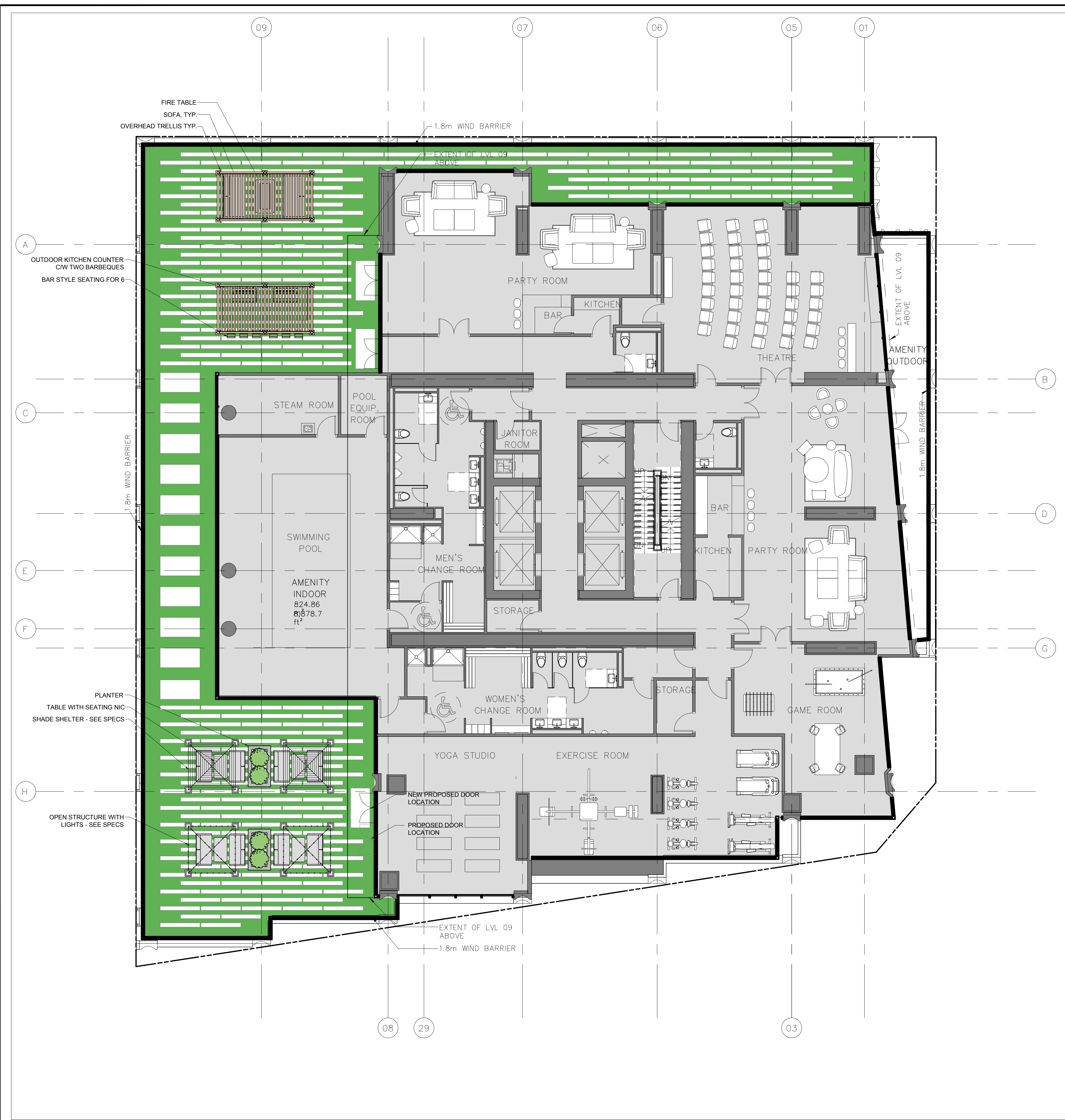
1 LEVEL 4 ROOF TERRACE LANDSCAPE PLAN SCALE 1:100
