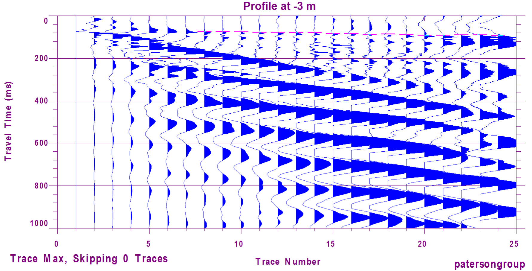
Figure 2 – Shear Wave Velocity Profile at Shot Location -3 m
