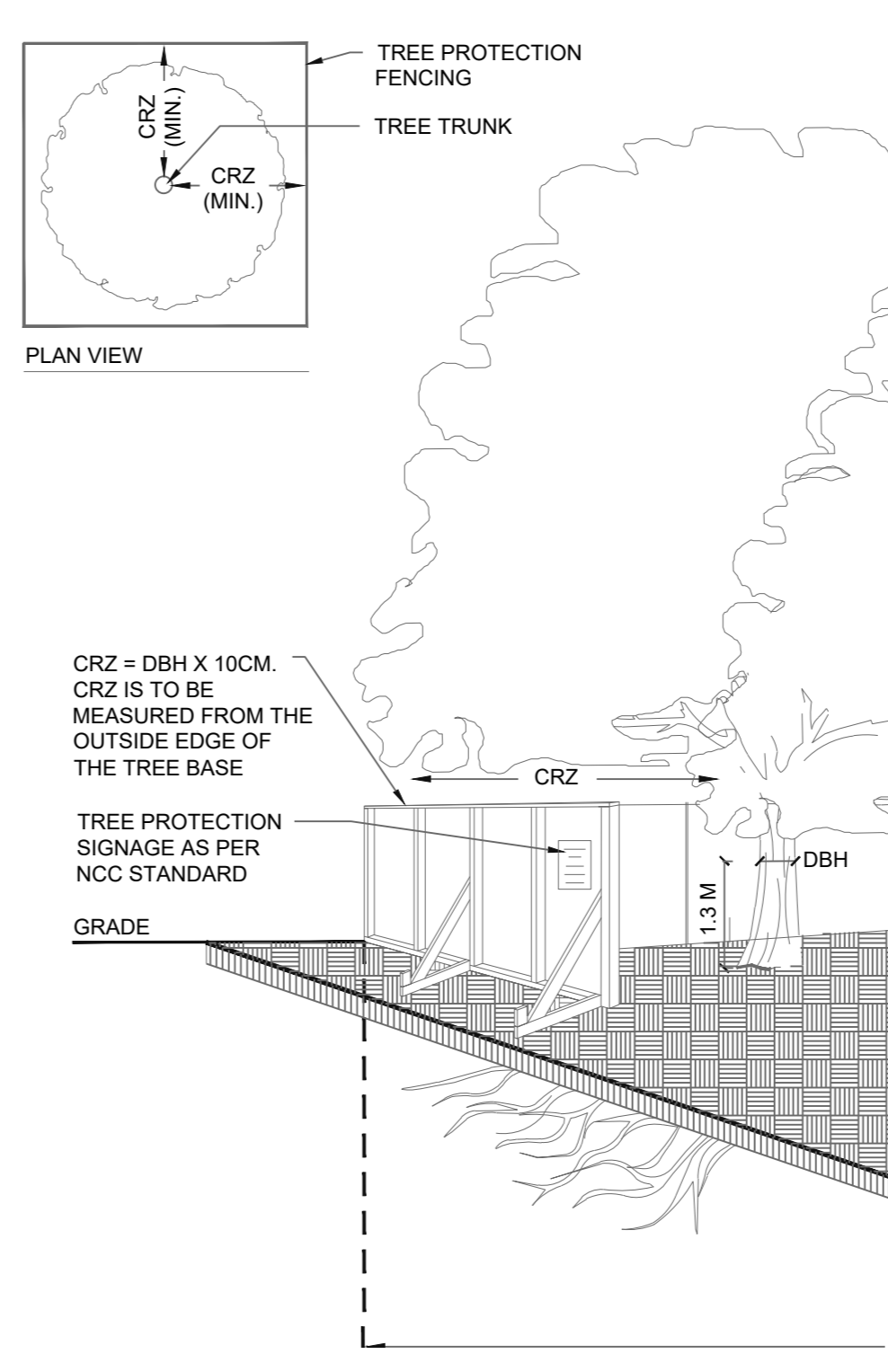
1 TREE PROTECTION FENCE DETAIL L2 N.T.S.
