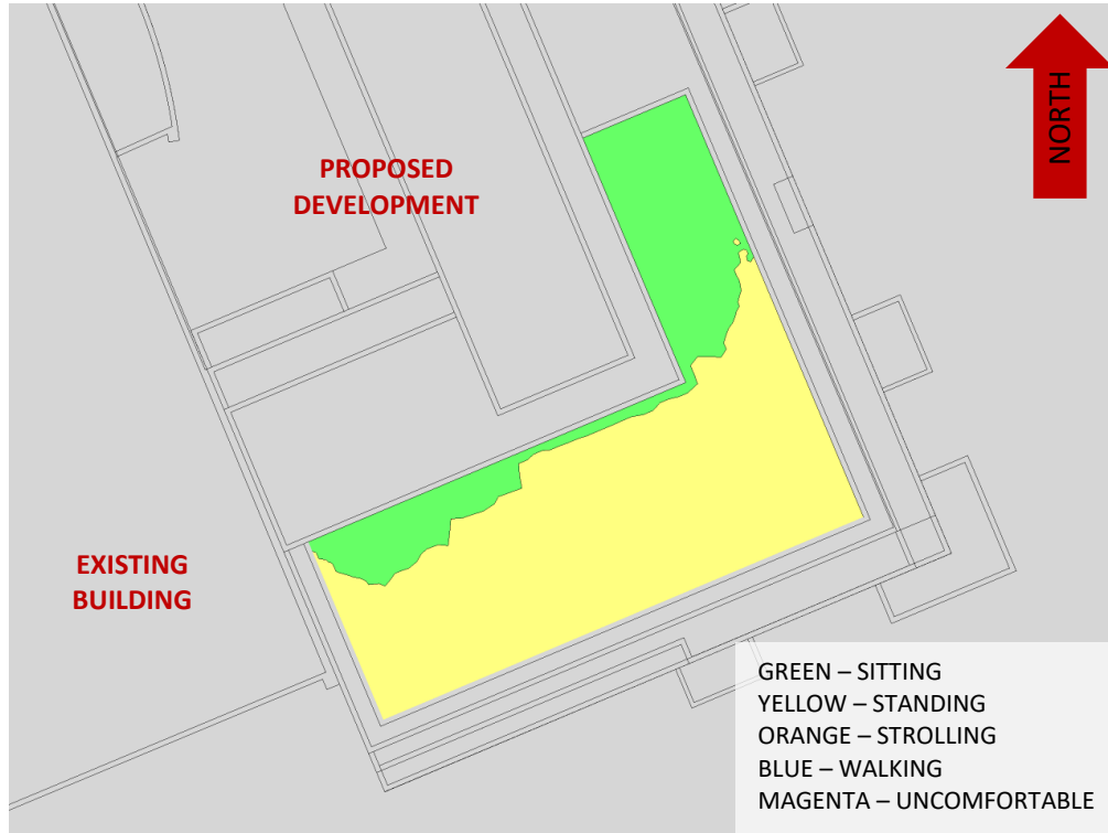
FIGURE 4C: AUTUMN – WIND COMFORT, AMENITY TERRACE (MECH PH, LOW DECK)
