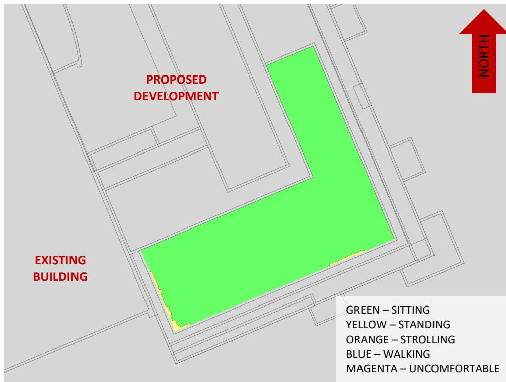
FIGURE 4A: SUMMER – WIND COMFORT, AMENITY TERRACE (MECH PH, LOW DECK)
