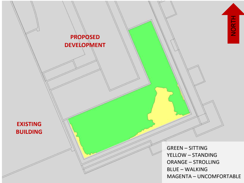
FIGURE 5A: TYPICAL USE PERIOD – WIND COMFORT, AMENITY TERRACE (MECH PH)
