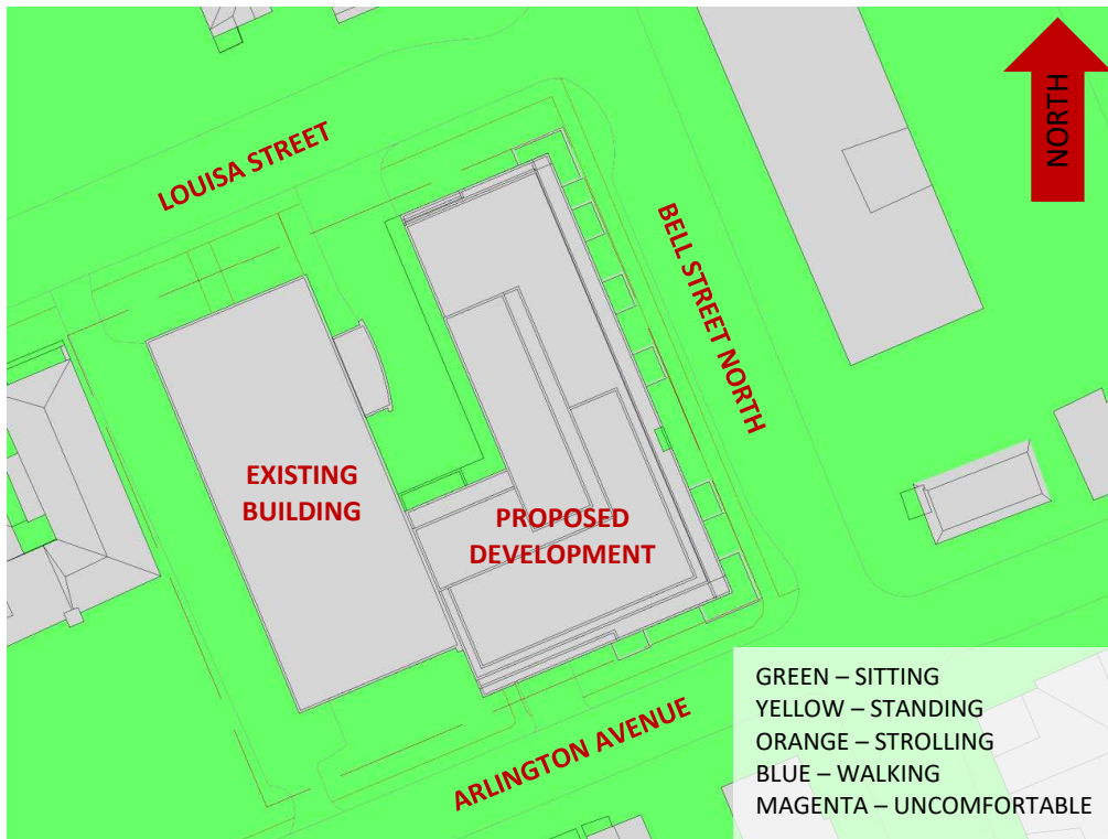
FIGURE 3B: SUMMER – WIND COMFORT CLASSES, GRADE LEVEL
