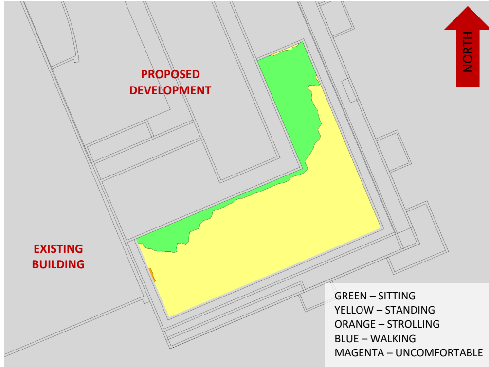
FIGURE 4A: SPRING – WIND COMFORT, AMENITY TERRACE (MECH PH, LOW DECK)
