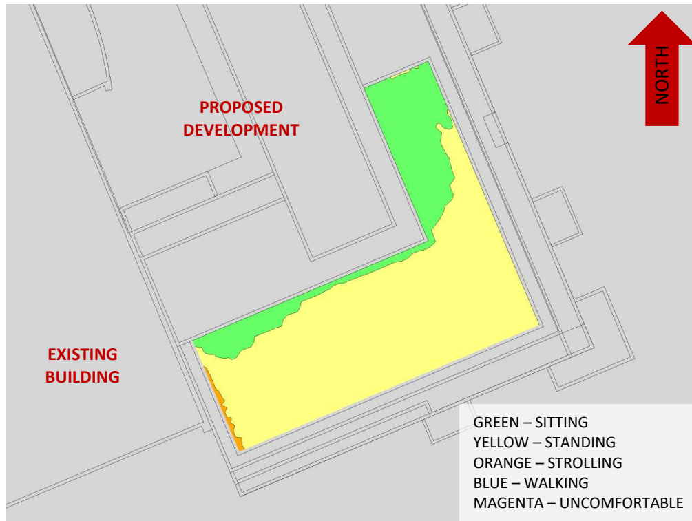
FIGURE 4D: WINTER – WIND COMFORT, AMENITY TERRACE (MECH PH, LOW DECK)
