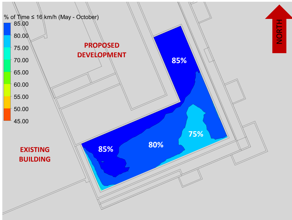
FIGURE 5B: TYPICAL USE PERIOD – PERCENTAGE OF TIME SUITABLE FOR SITTING (MECH PH)
