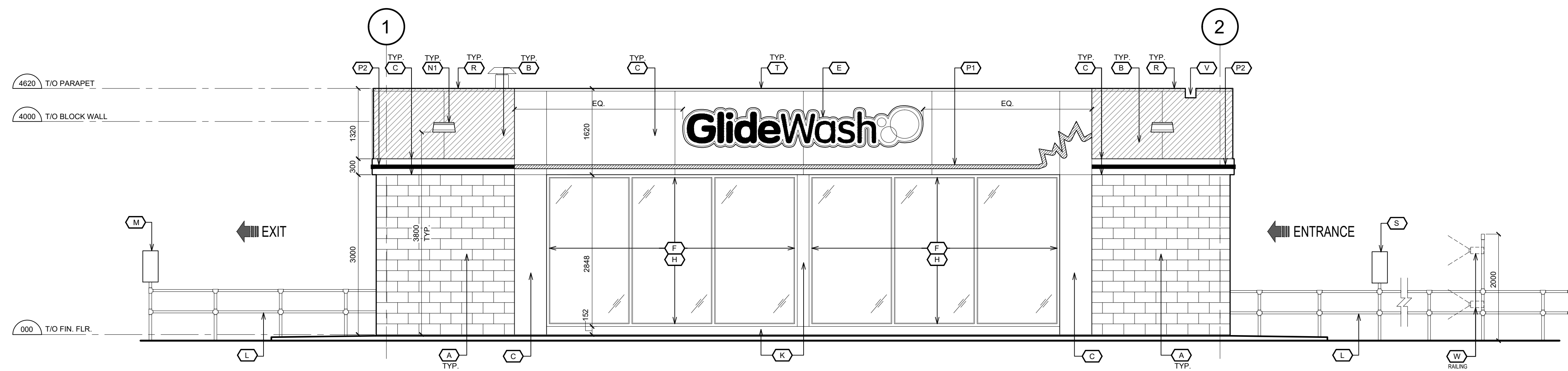
1 SOUTH ELEVATION
