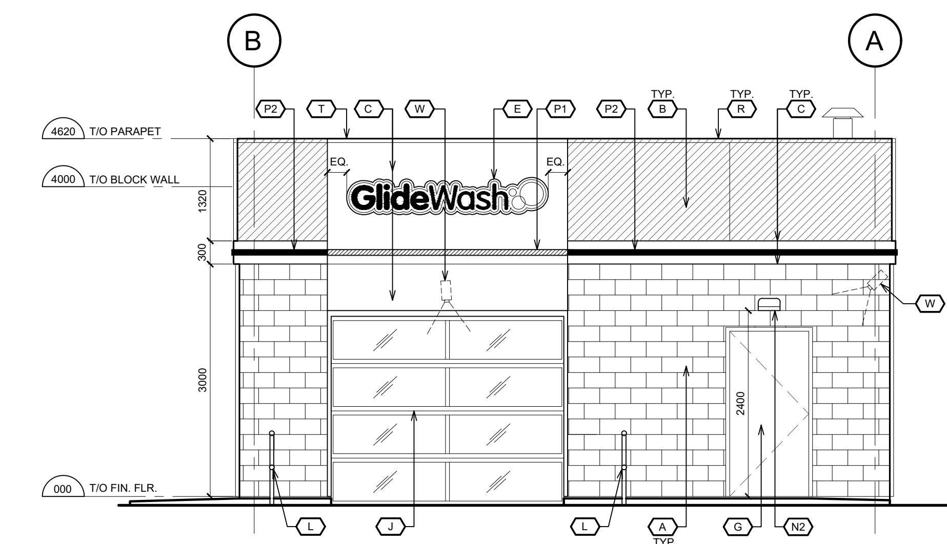
3 EAST ELEVATION
