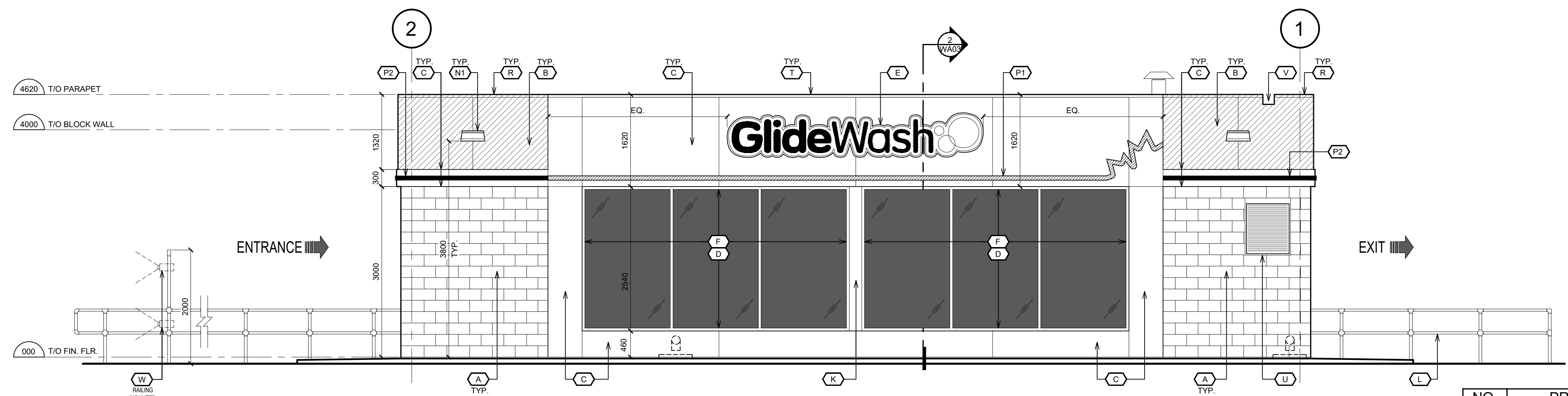
2 NORTH ELEVATION
