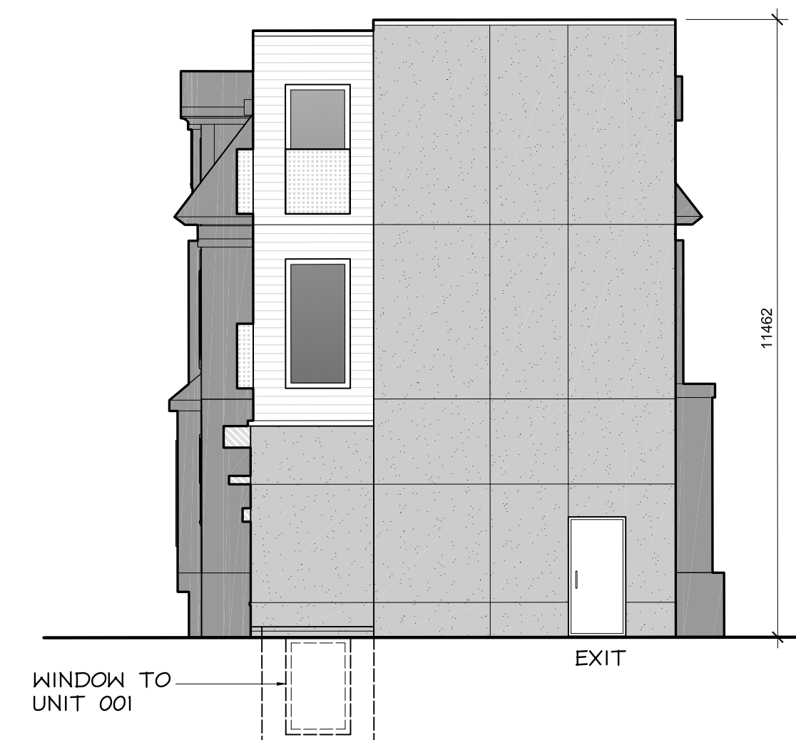
4 A200 NORTH ELEVATION 1:100
