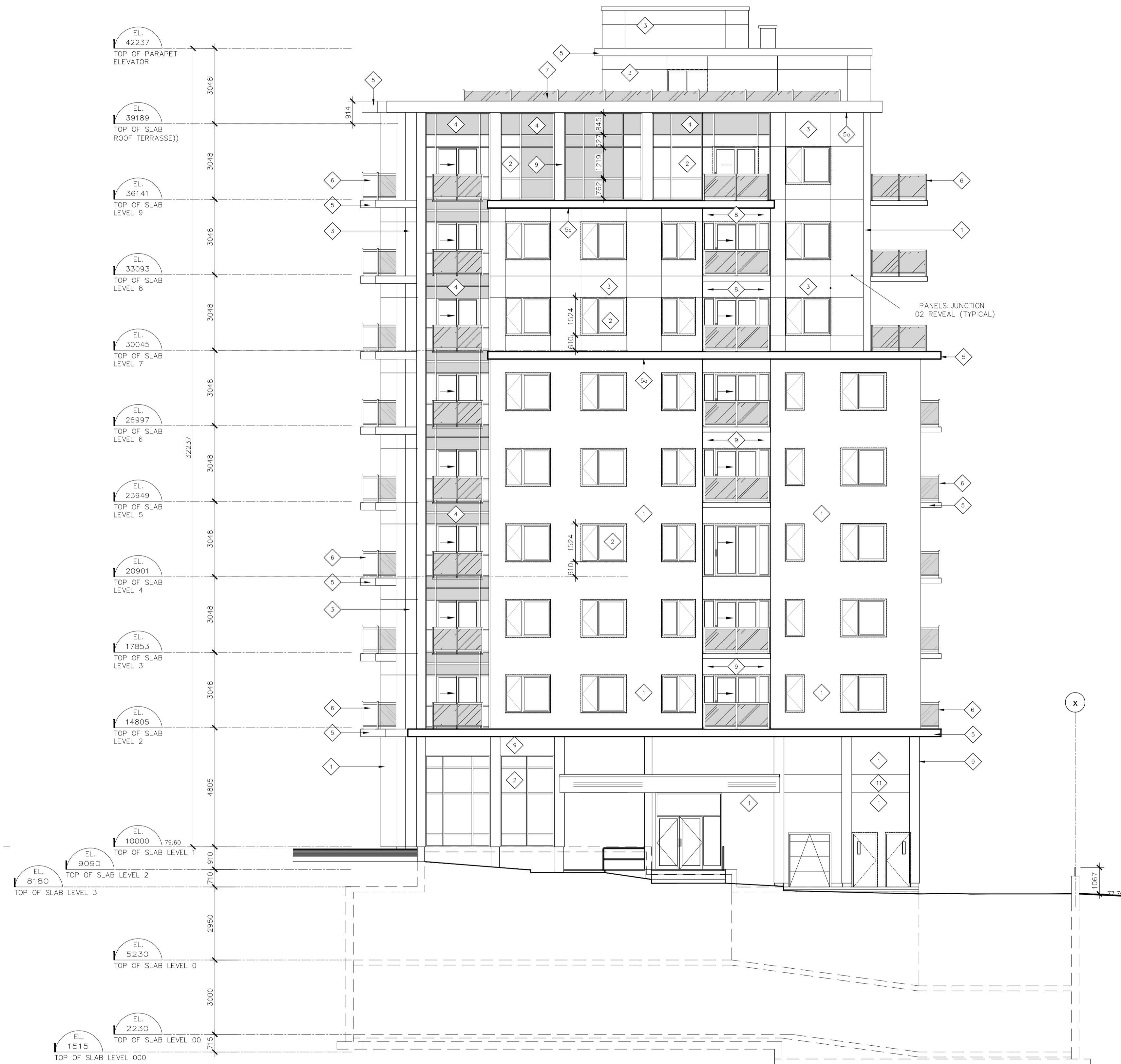
02 ELEVATION - LATERAL RIGHT 1:100
