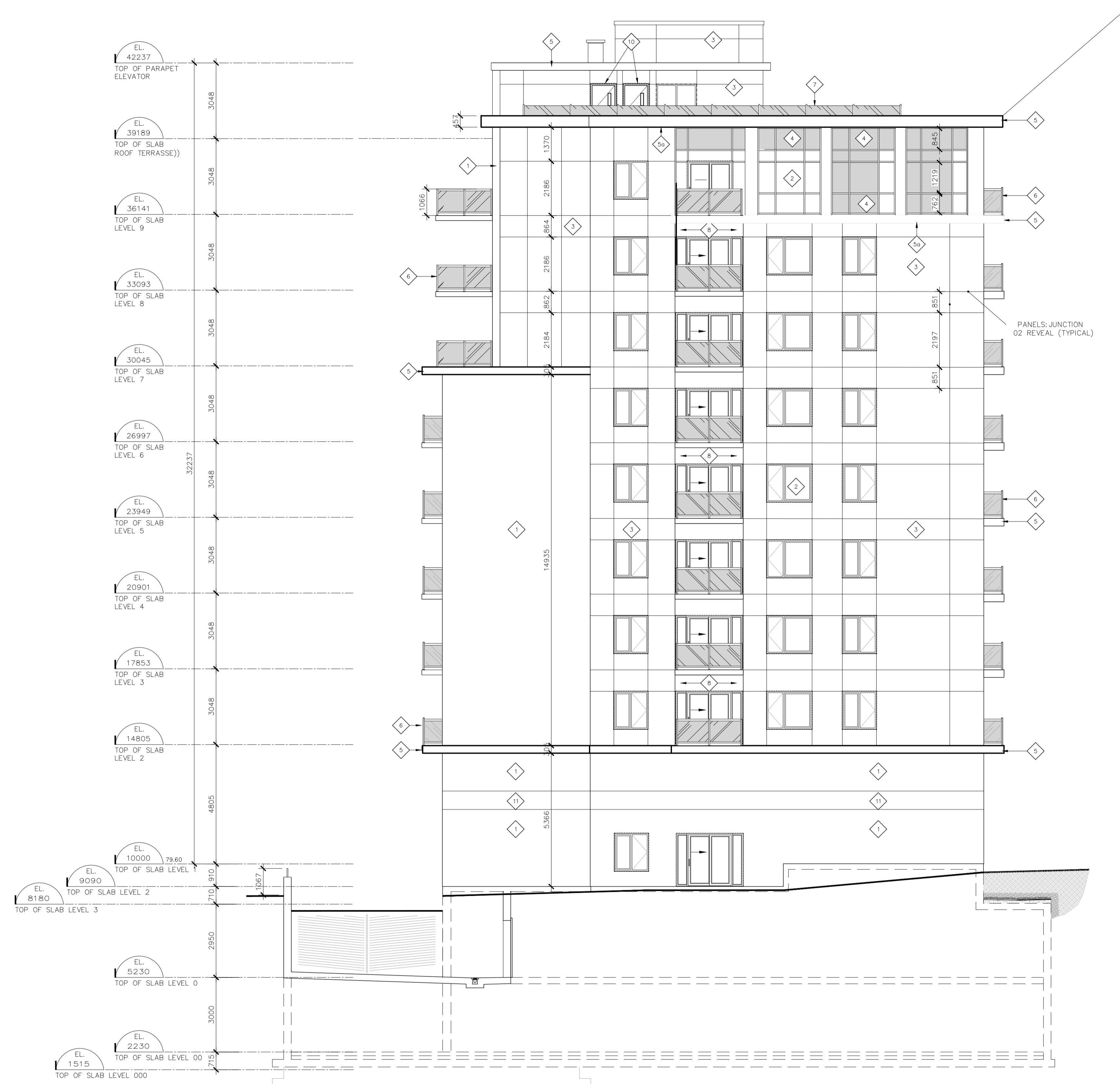
03 ELEVATION - LATERAL LEFT 1 : 100
