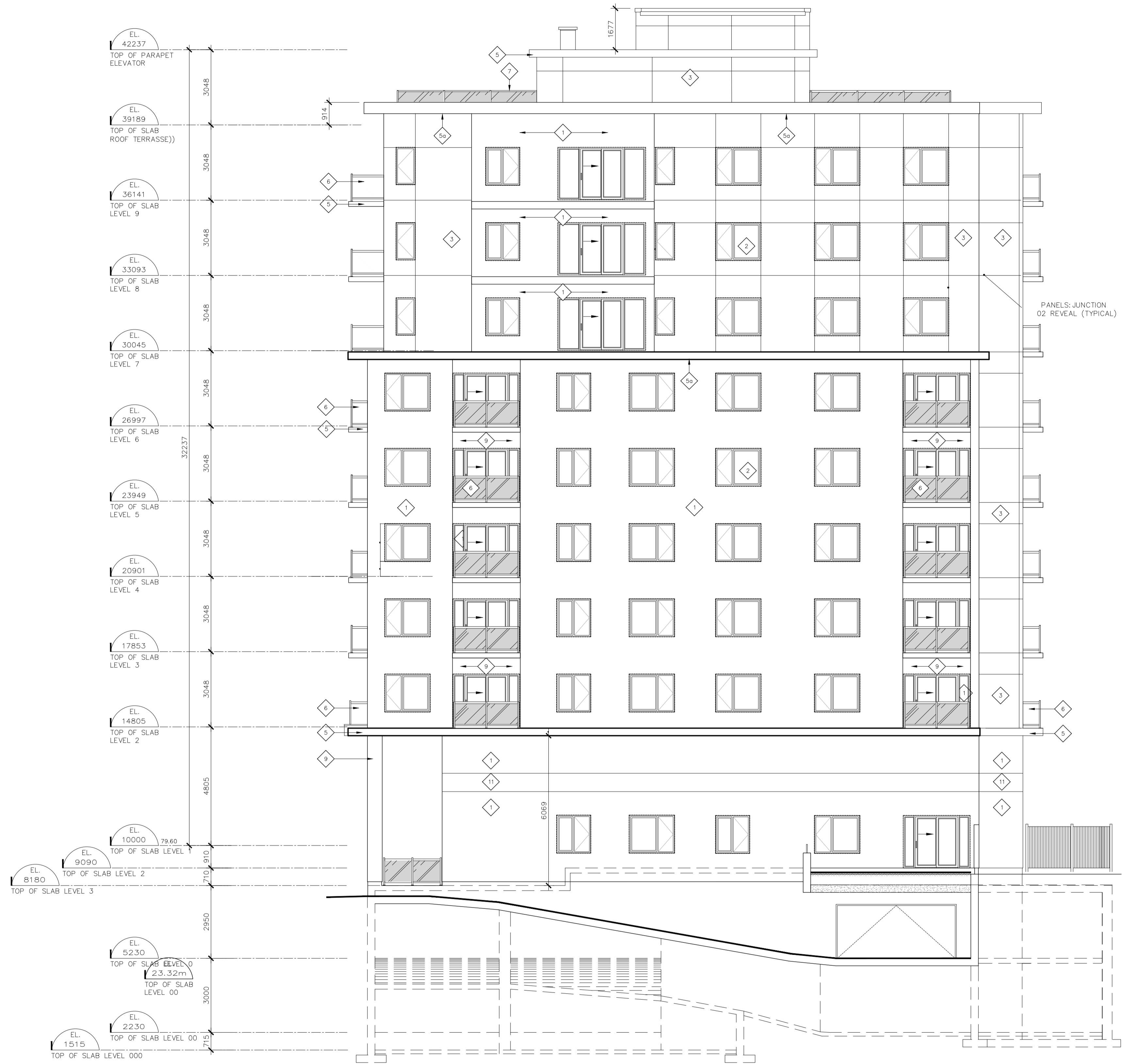
04 REAR ELEVATION 1:100
