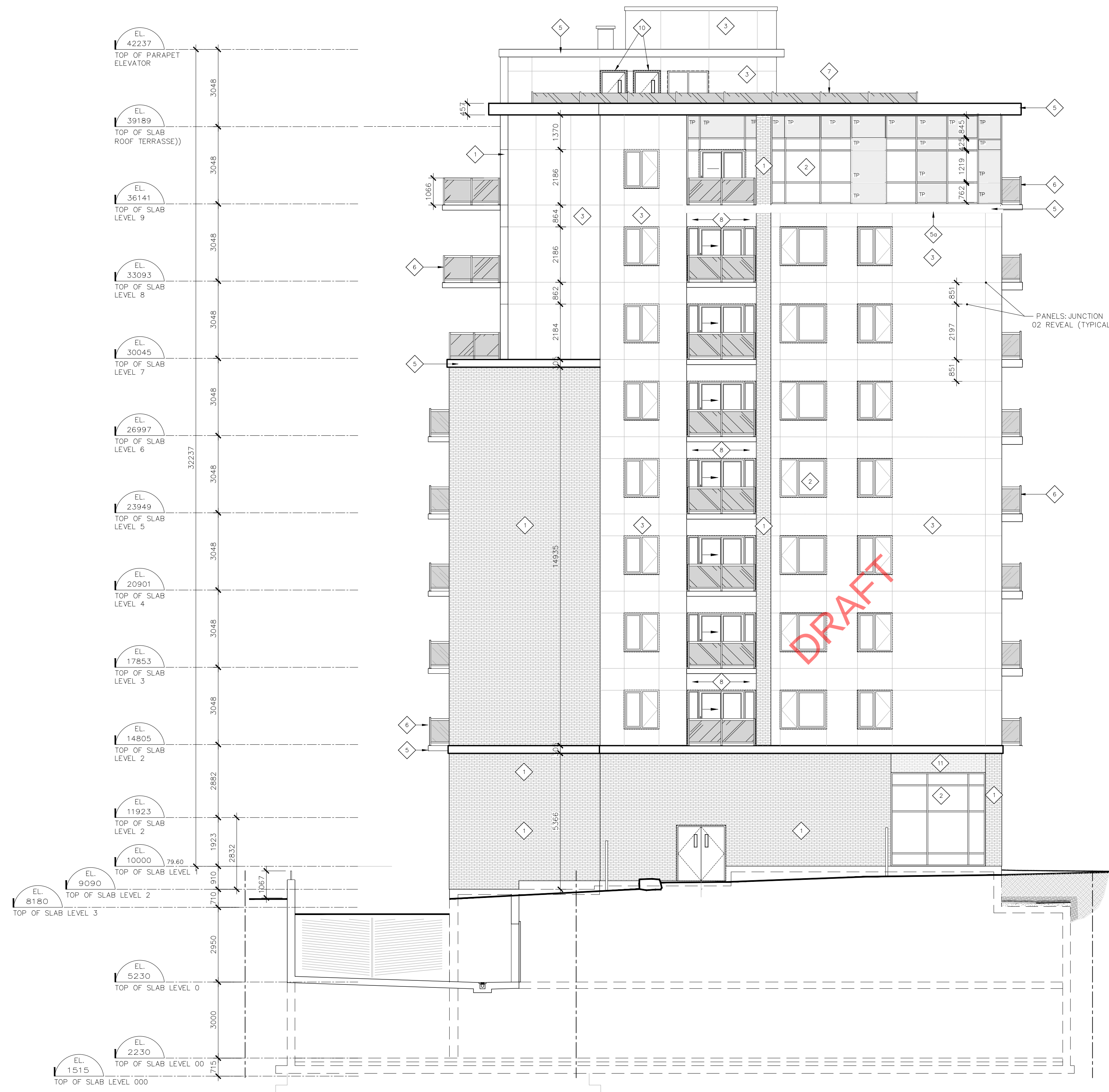
03 WEST ELEVATION 1 : 100
