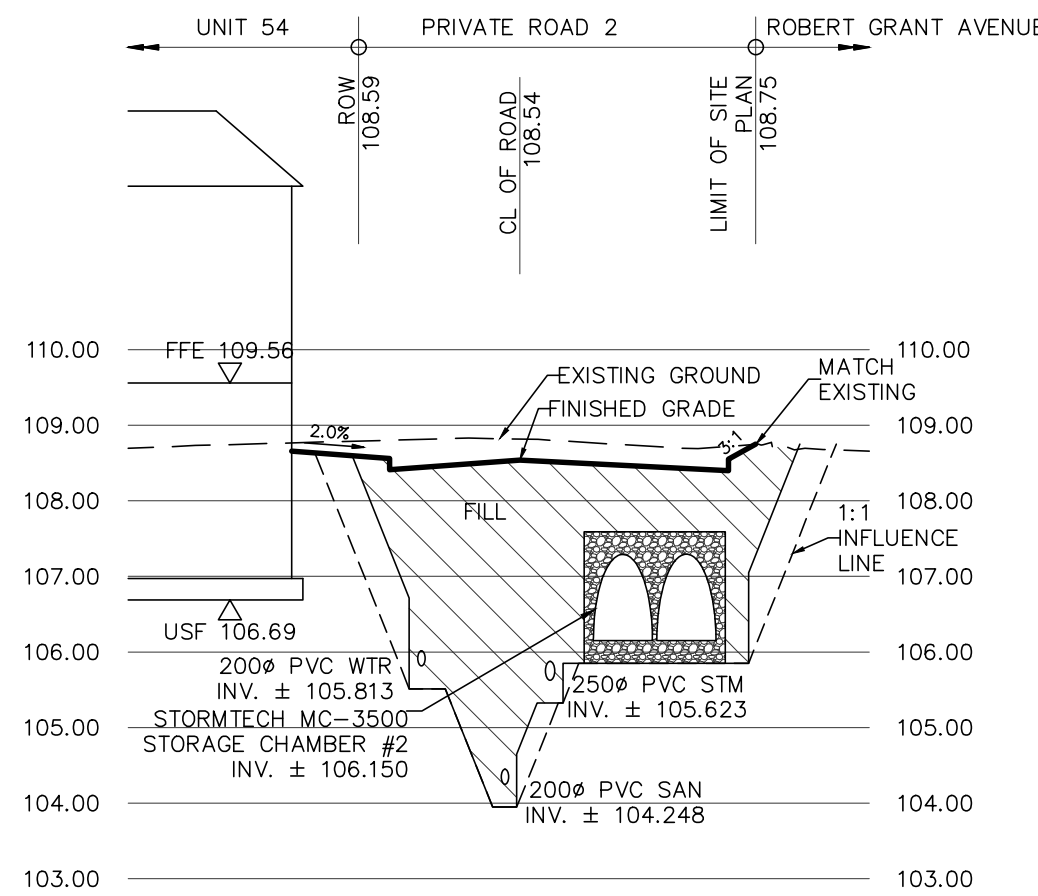
SECTION 2-2 SCALE HOR: 1:250 VER: 1:100
