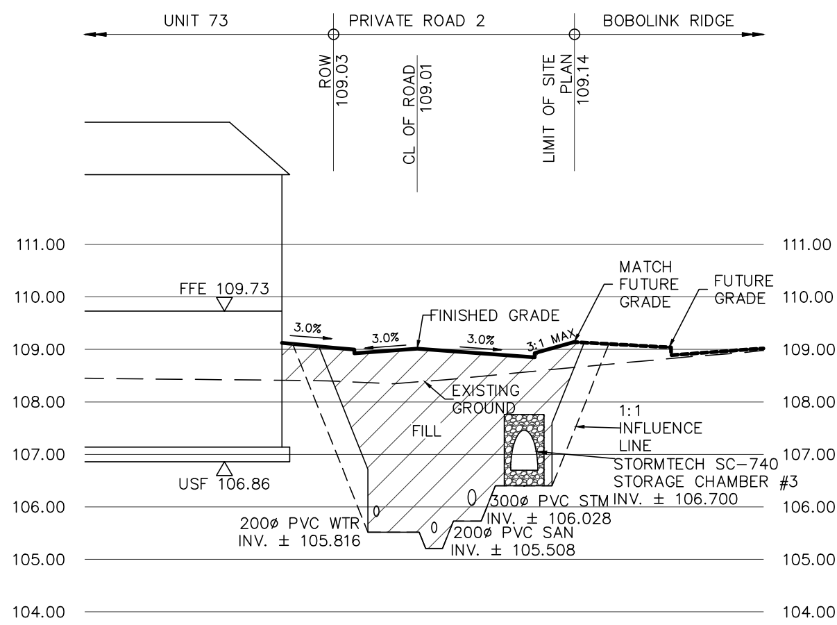
SECTION 3-3 SCALE HOR: 1:250 VER: 1:100
