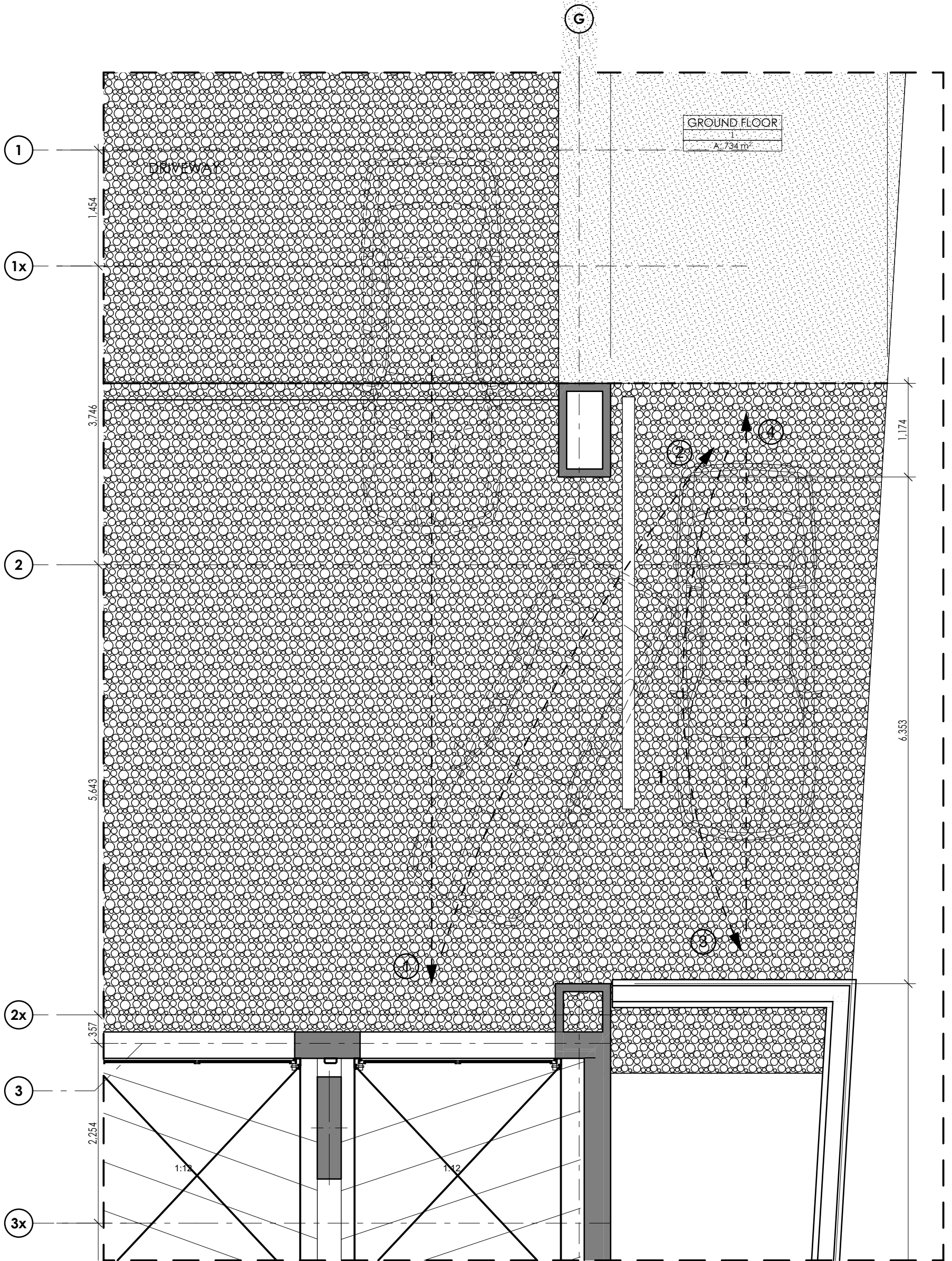
1 DSK - 01 ACCESS TO PARKING STALL 1 DSK-01 SCALE: 1:50
