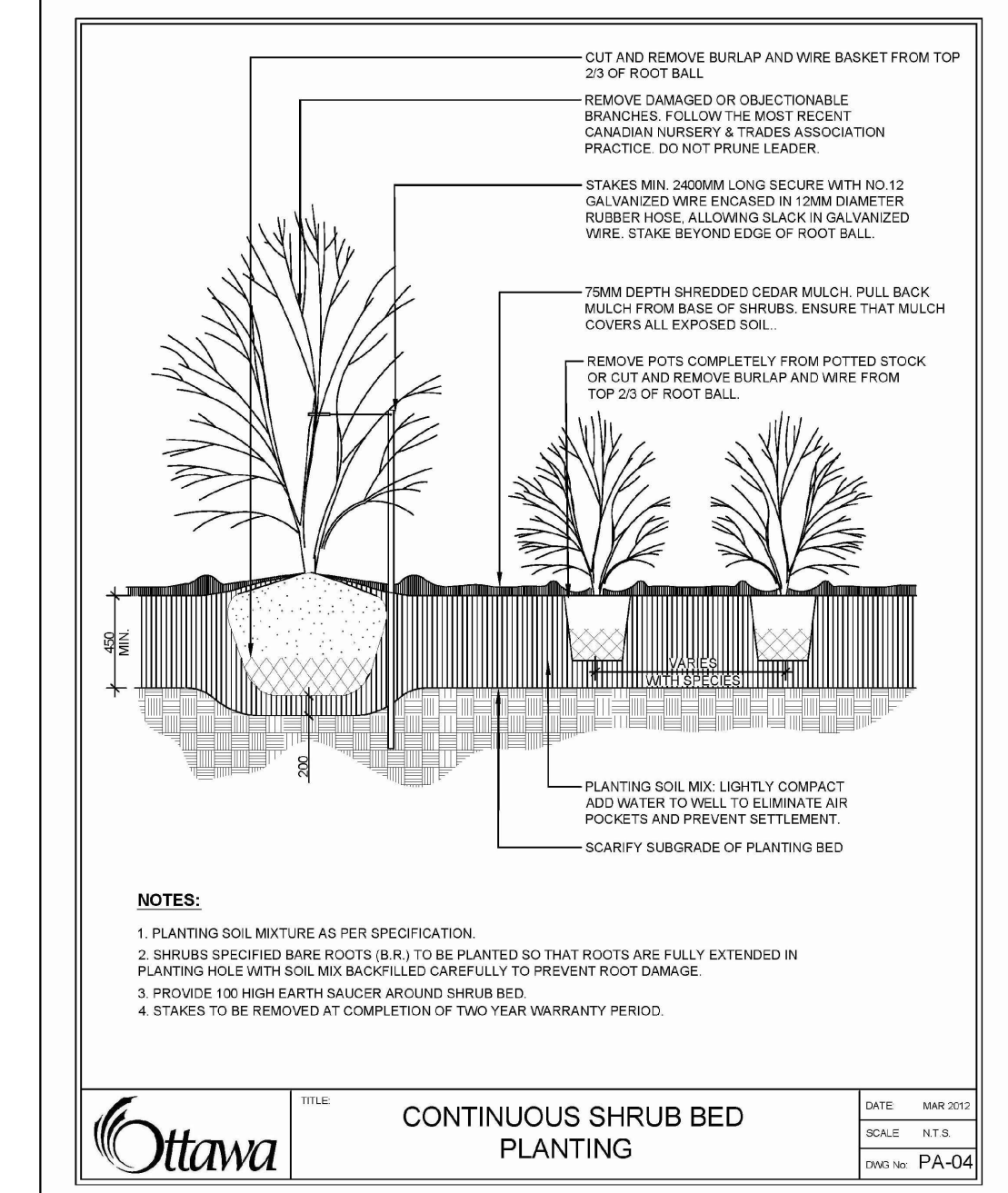
3 SHRUB BED PLANTING SCALE: NTS
