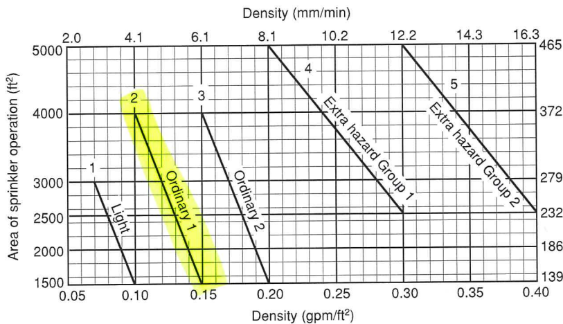
Figure 7-2.3.1.2 Area/density curves.
