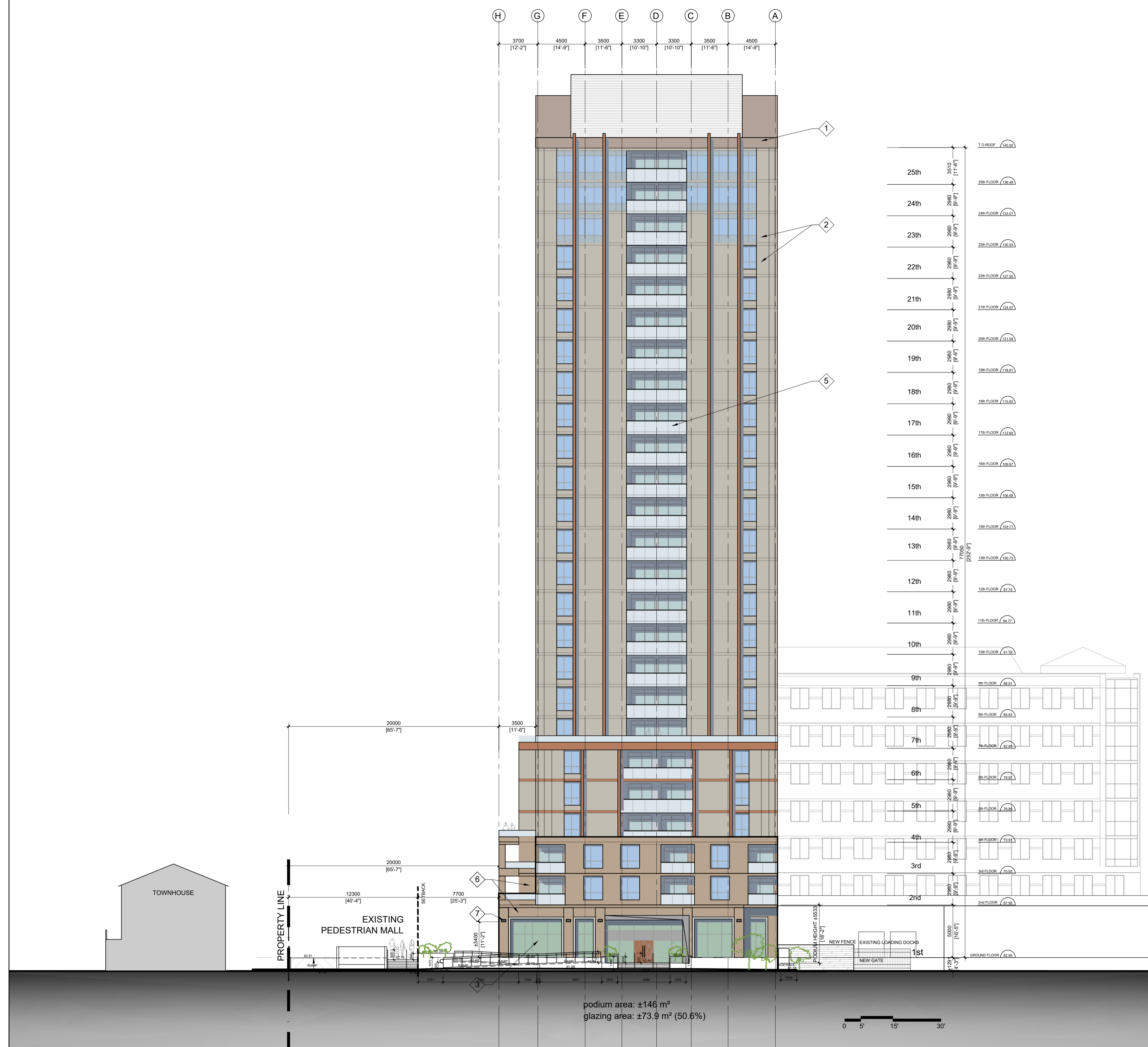
1 EAST ELEVATION A-203 SCALE 1:200
