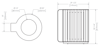
1 WASTE RECEPTACLE BY MAGLIN N.T.S.
