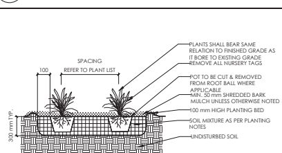
7 PERENNIAL AND GRASSES PLANTING N.T.S.
