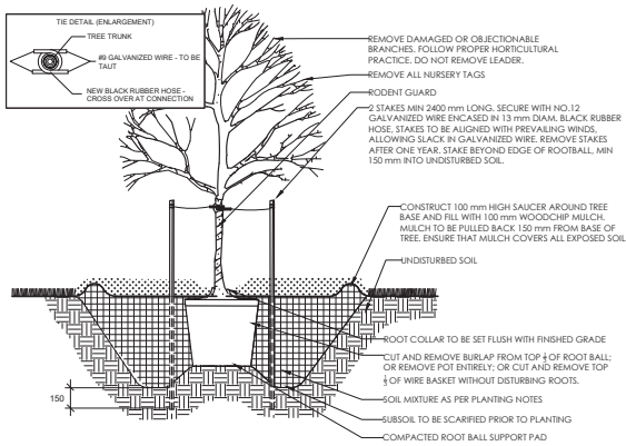
4 DECIDUOUS TREE PLANTING N.T.S.
