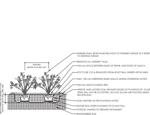
6 SHRUB PLANTING N.T.S.
