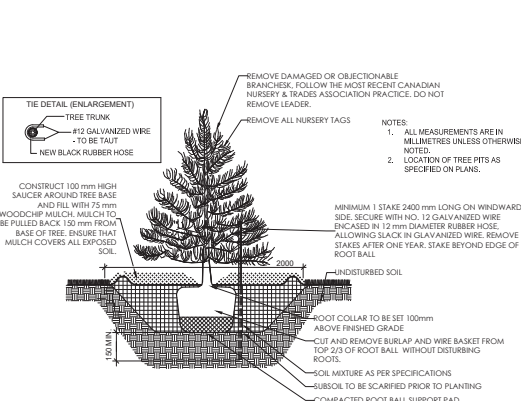
5 CONIFEROUS TREE PLANTING DETAIL N.T.S.
