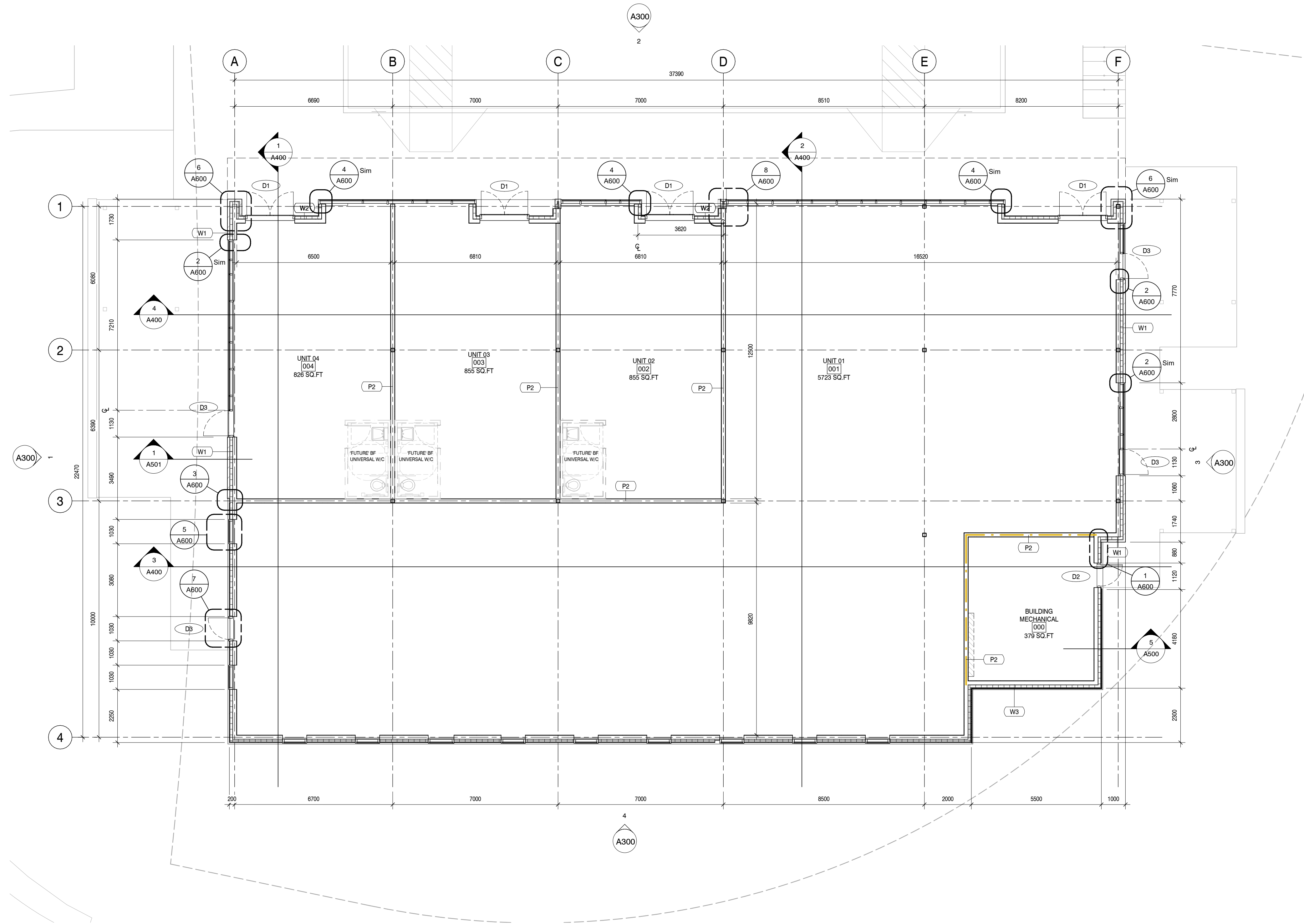
1 GROUND FLOOR PLAN A100 1:100
