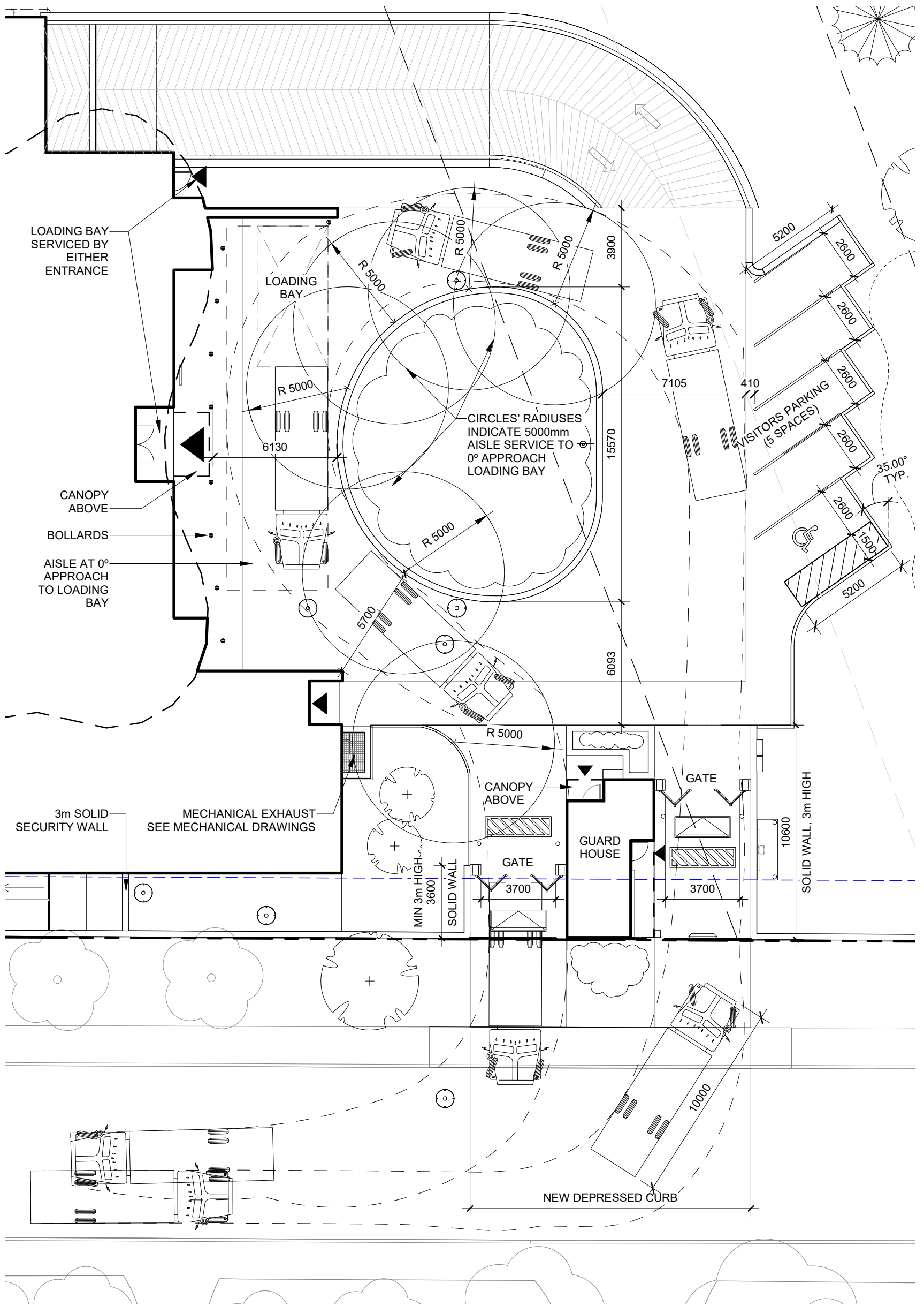
SITE PLAN - TURNING RADIUSES SCALE: 1 : 200
