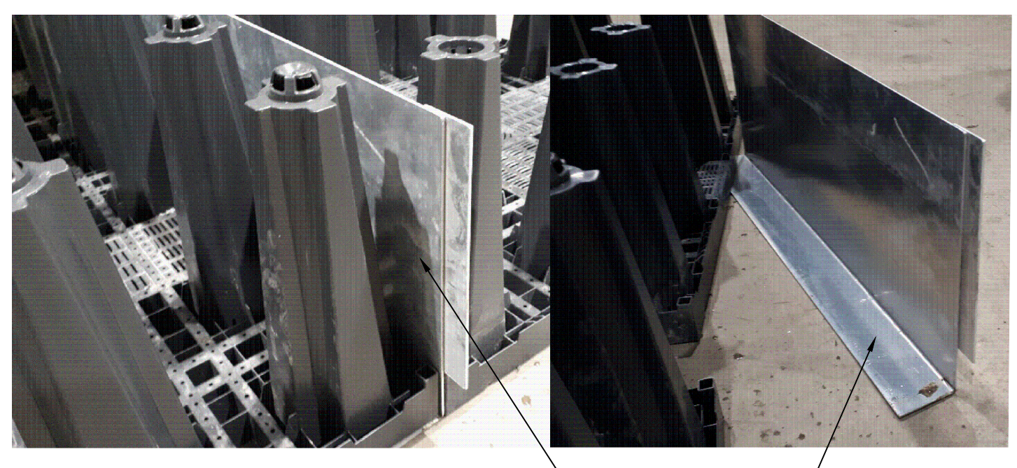
STANDARD TREATMENT ROW DETAIL (WHERE APPLICABLE)
