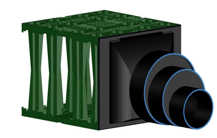
STANDARD ADAPTER PANEL WITH DIA 450 AND 525
