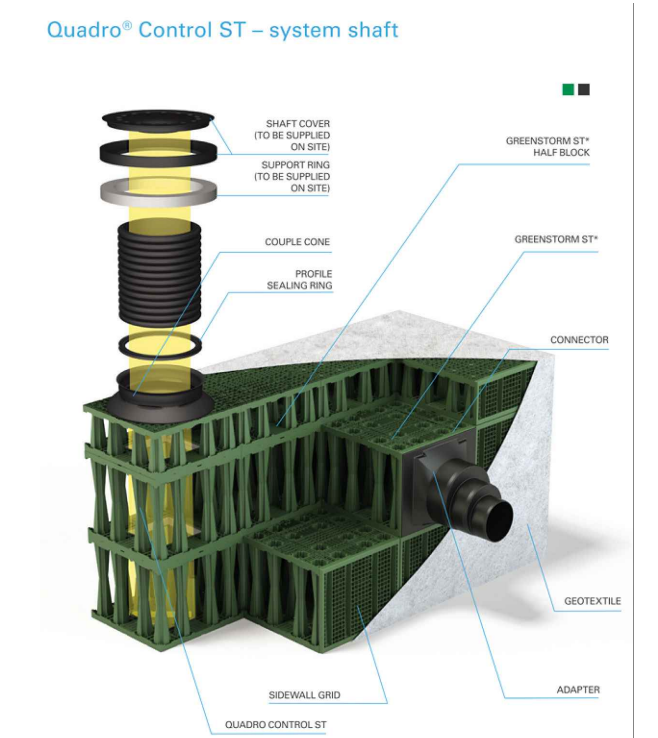
GREENSTORM ACCESS QUADRO DETAIL (WHERE APPLICABLE)
