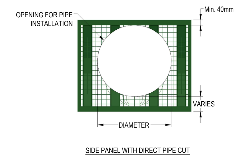
STANDARD SIDE PANEL WITH DIRECT PIPE CUT
