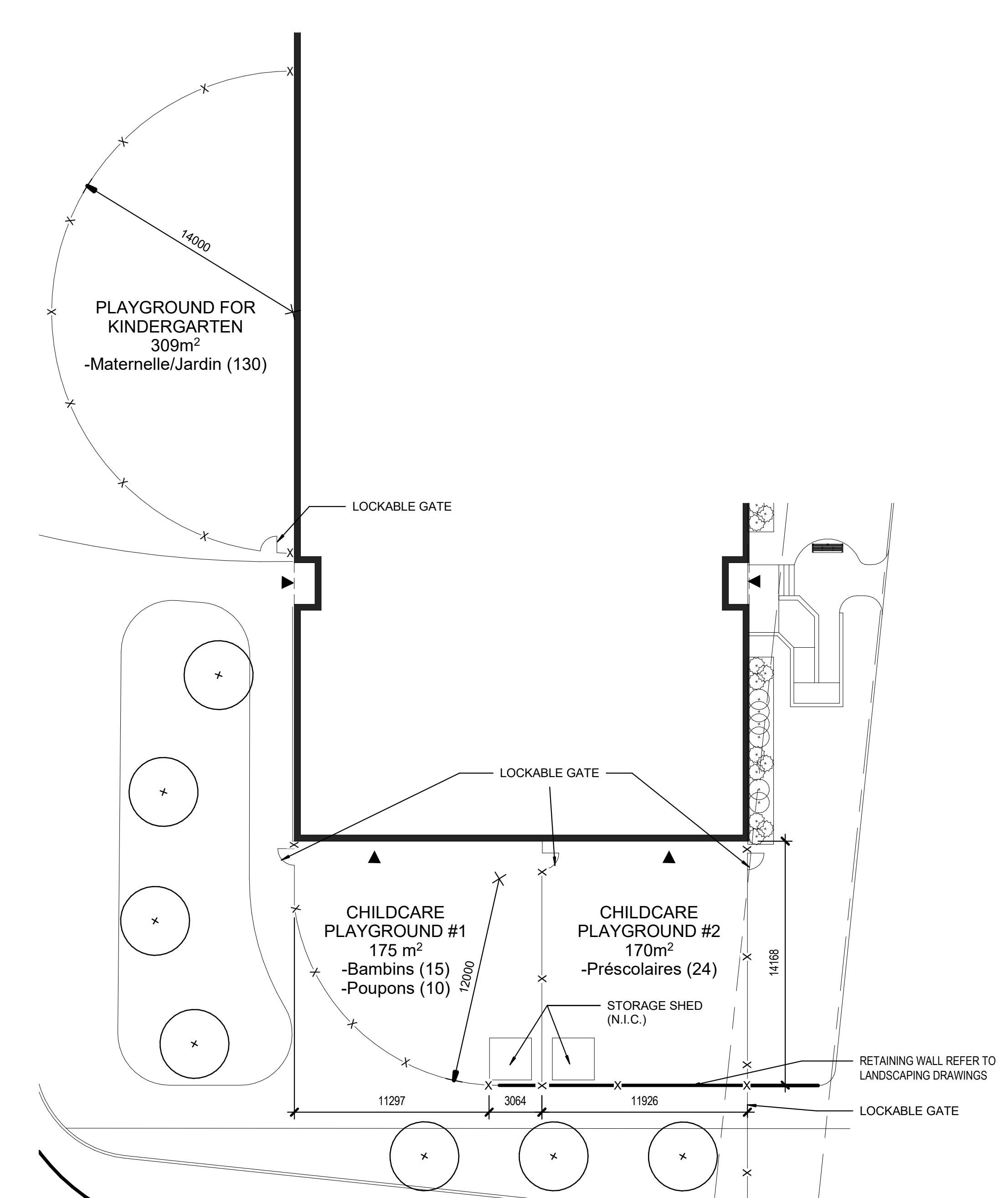
ENLARGED DAYCARE SITE PLAN 1:200
