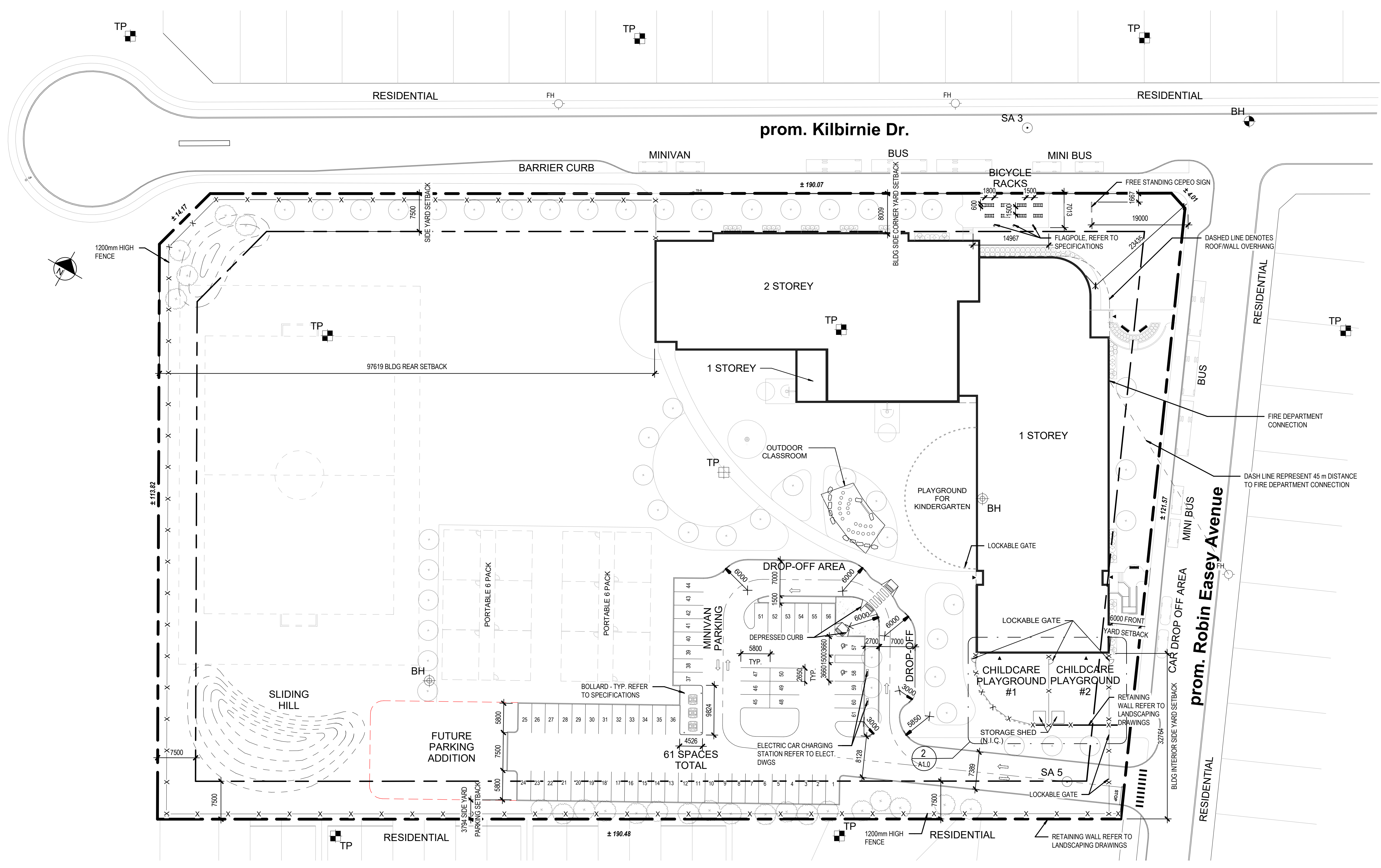
GENERAL SITE PLAN 1:400
